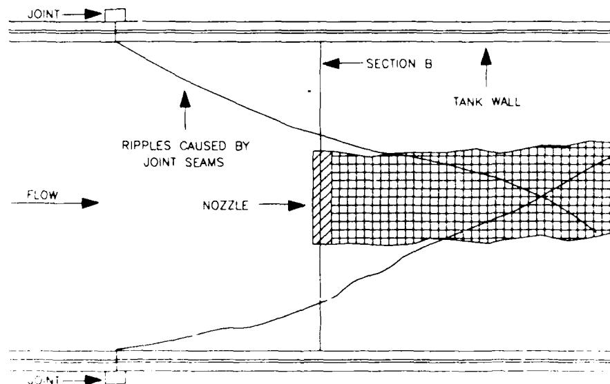
Figure 8. Location of nozzle during testing
