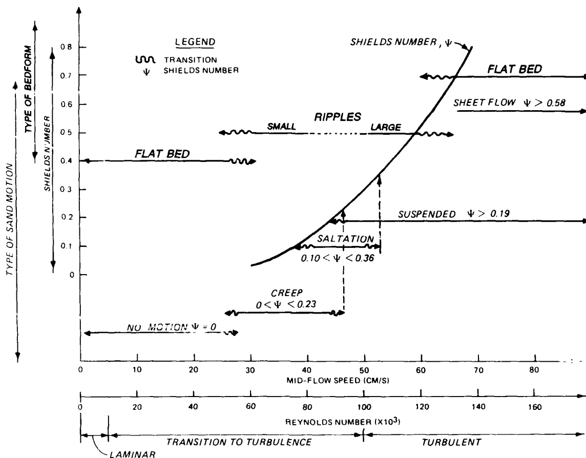
Figure 22. Bed configuration and sand movement as a function of midflow speed, Reynolds number, and Shields number
