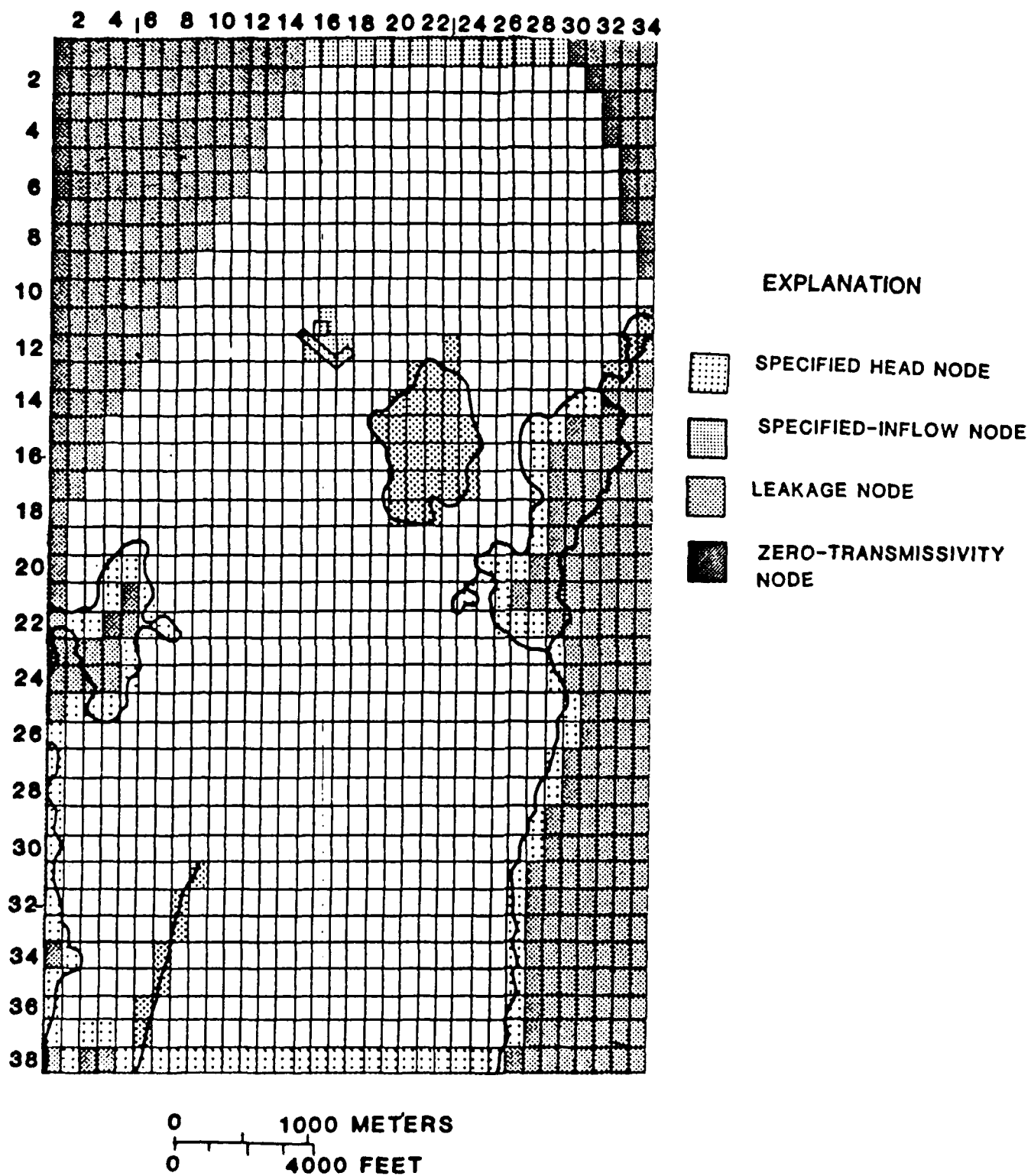
Figure 56. Grid for the Random Walk Simulation of the Otis Sewage Plume.
