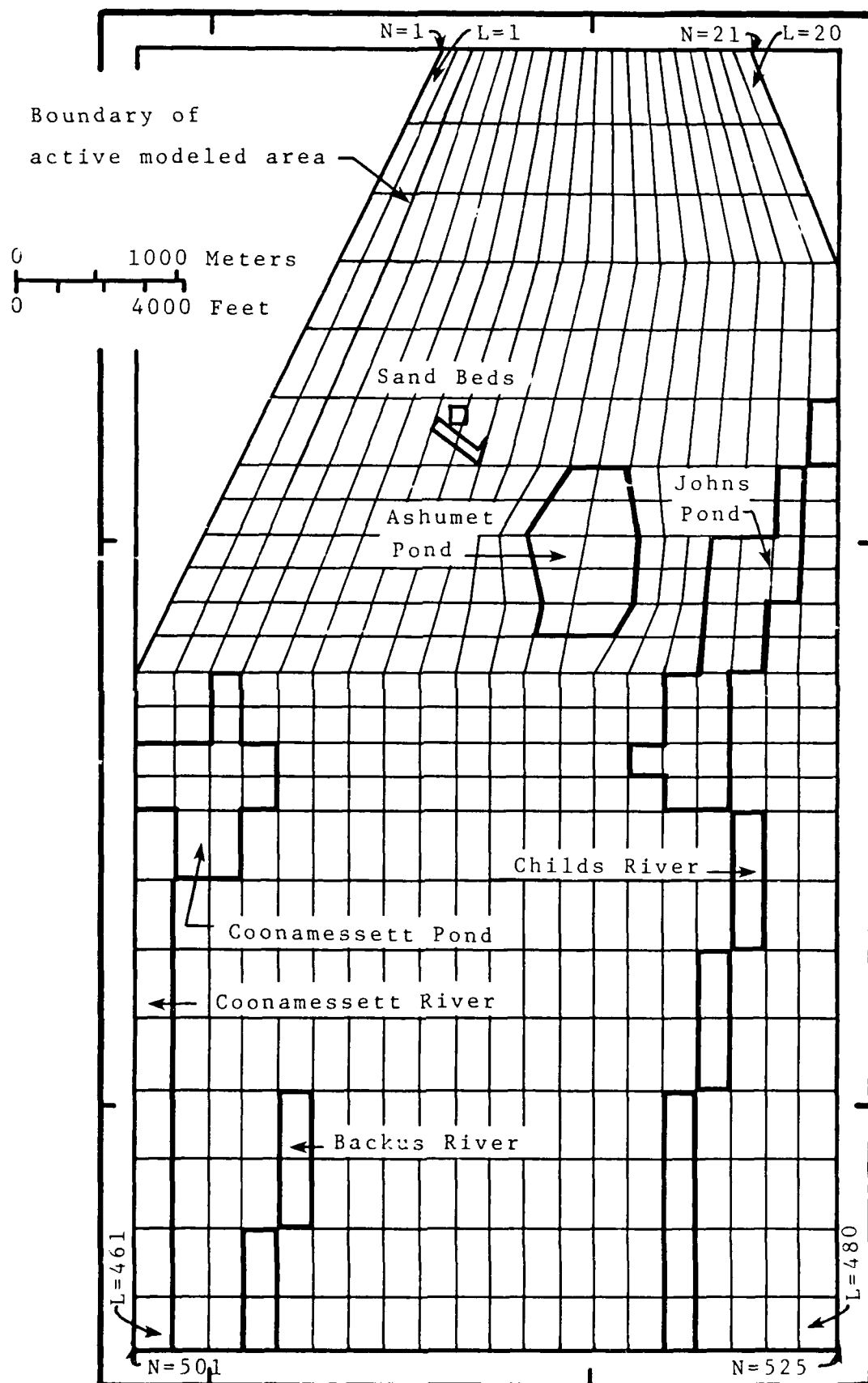
Figure 91. SUTRA-82 Grid Chosen for the Otis ANGB Sewage Plume.
