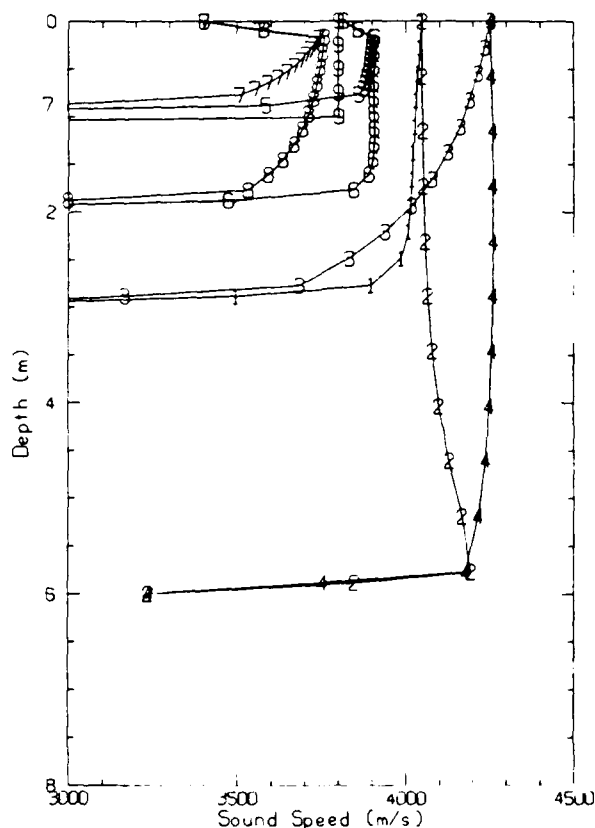
Figure 4. Sound speed profiles used for simulations. The following parameters for each SSP are given in the order of type of ice, thickness, and surface temperature: (1) multiyear, 3 m, -22.5^{\circ}\text{C} ; (2) multiyear, 6 m, -22.5^{\circ}\text{C} ; (3) multiyear, 3 m, -5^{\circ}\text{C} ; (4) multiyear, 6 m, -5^{\circ}\text{C} ; (5) first year, 1 m, -22.5^{\circ}\text{C} ; (6) first year, 2 m, -22.5^{\circ}\text{C} ; (7) first year, 1 m, -5^{\circ}\text{C} ; (8) first year, 2 m, -5^{\circ}\text{C} ; and (9) idealized profile with zero gradient in ice and water.
