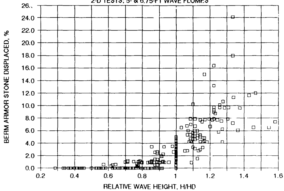
Figure 19. Percentage of toe berm armor stone displaced versus relative wave height (2-D tests)
