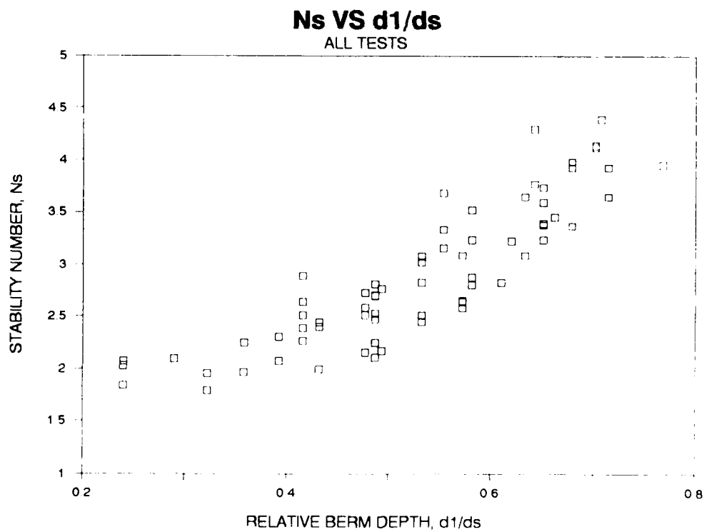
Figure 12. Stability number versus relative berm depth for all toe berm stone tests which produced design data
