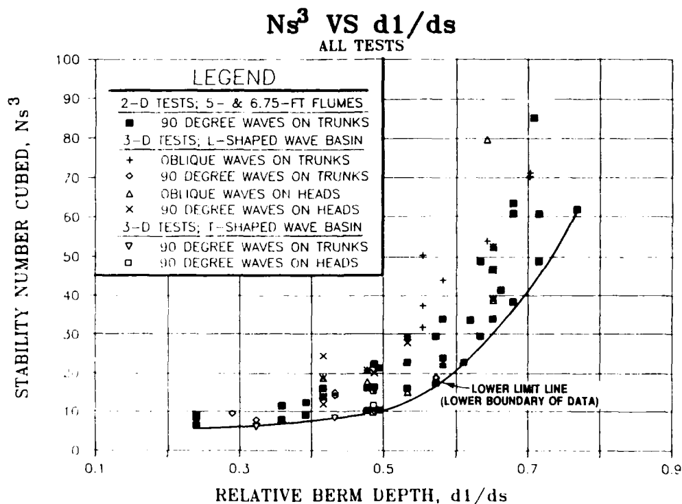
Figure 14. Stability number cubed versus relative berm depth for all toe berm stone tests which produced design data
