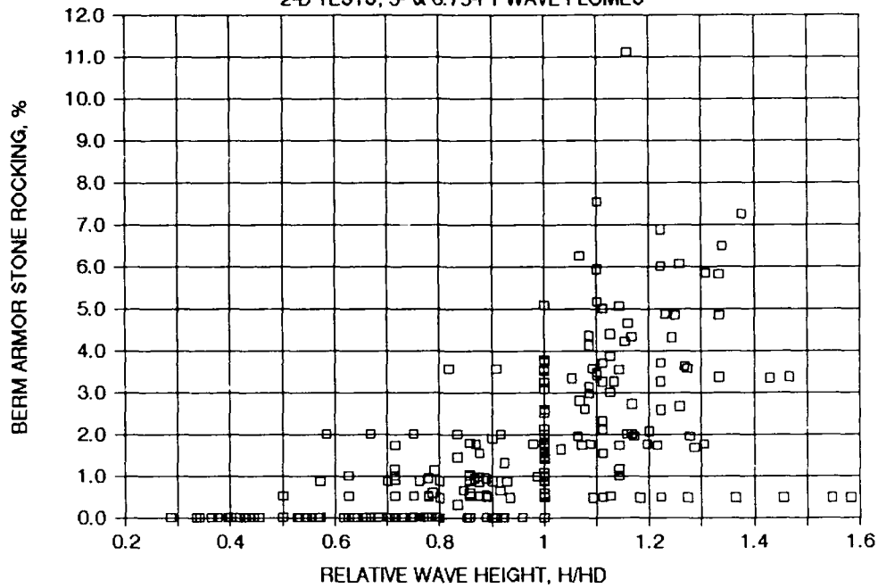
Figure 18. Percentage of toe berm armor stone which exhibited rocking versus relative wave height (2-D tests)
