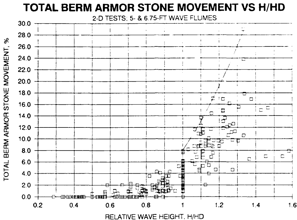
Figure 20. Total percentage of berm armor stone showing any type of movement (rocking or displacement) versus relative wave height (2-D tests)
