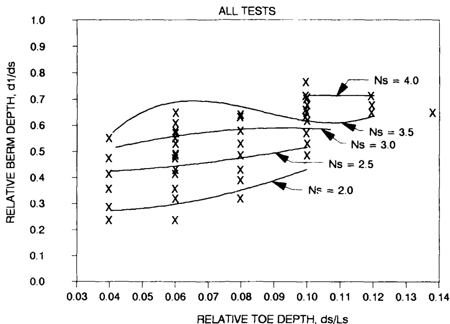
Figure 13. Contours of equal stability number for the ranges of relative berm depth and relative water depth at toe which produced design data for toe berms
