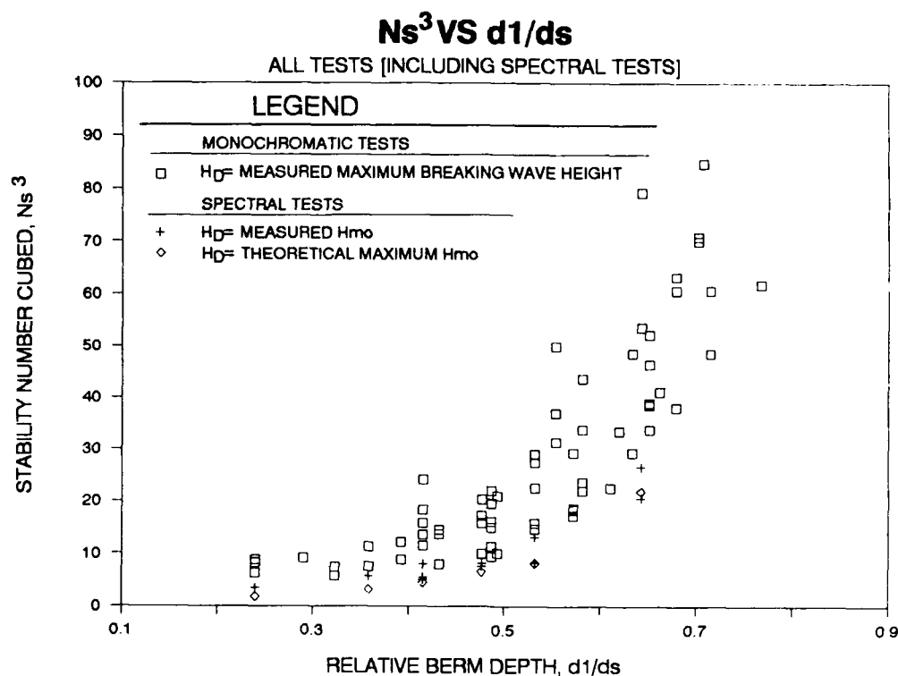
Figure 17. Stability number cubed versus relative berm depth for all toe berm stone tests including spectral wave tests
