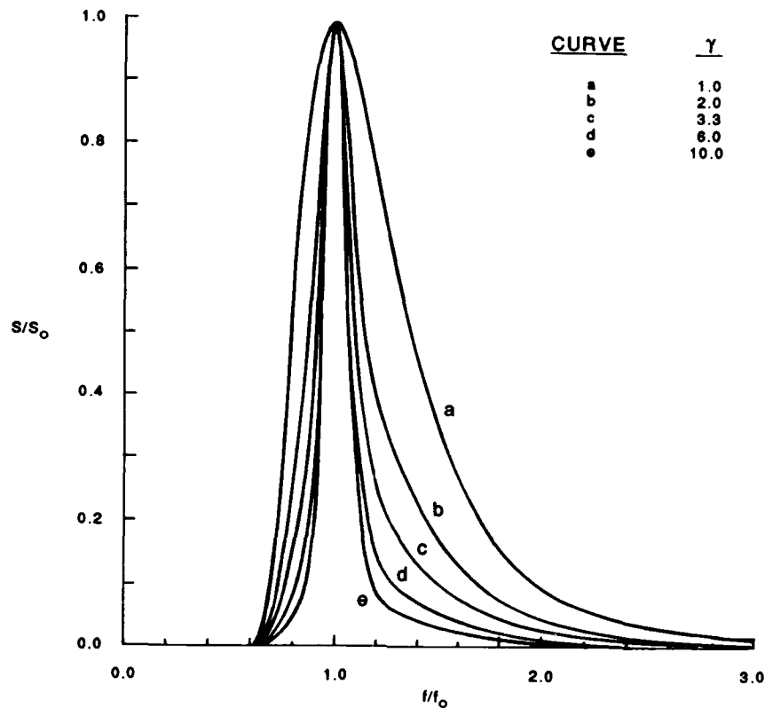
Figure 16. Five examples of JONSWAP spectra in dimensionless form (Case (a) is a Pierson-Moskowitz spectrum; Case (c) is the result of the JONSWAP experiment)
