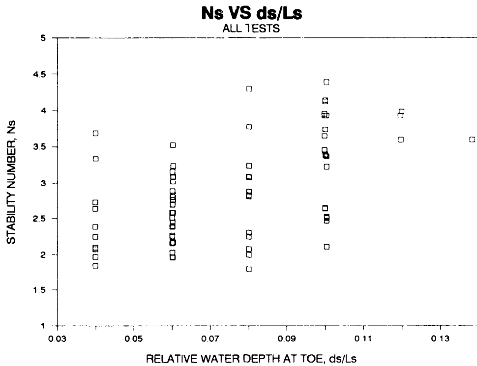
Figure 11. Stability number versus relative water depth at toe for toe berm stone tests which produced design data
