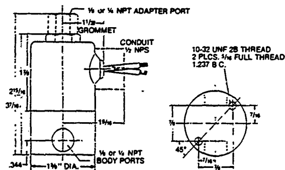
OUTLINE AND MOUNTING DIMENSIONS
