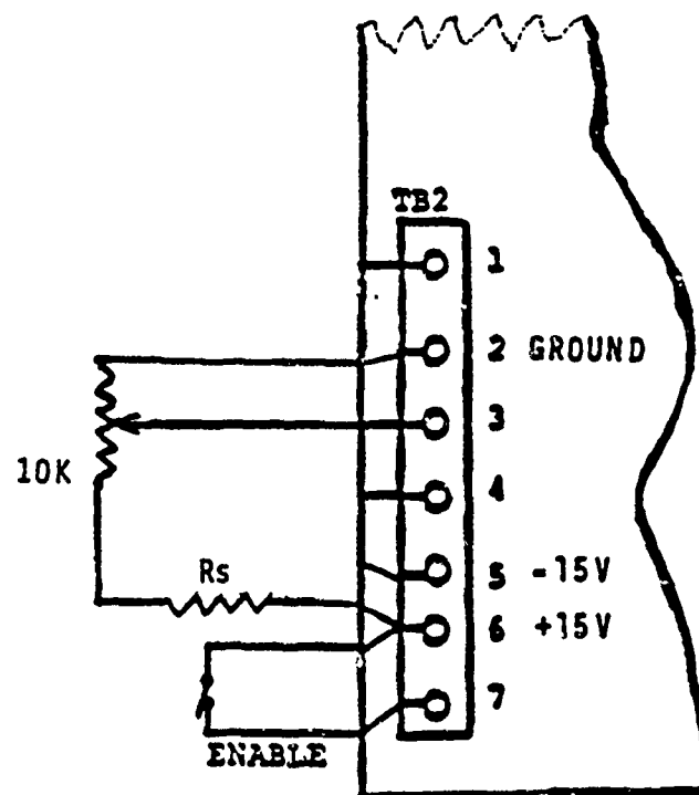
D. 1-direction control EMF Sensing
