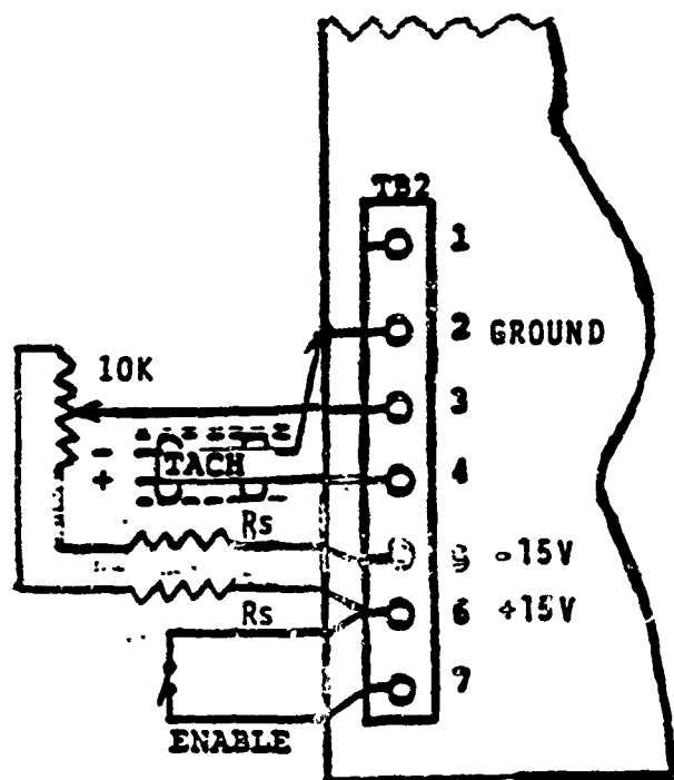
A. 2-direction control Tachometer Feedback
