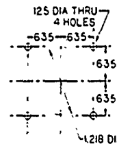
MOUNTING CUTOUT FOR SQ. SNAP-ON BEZEL
