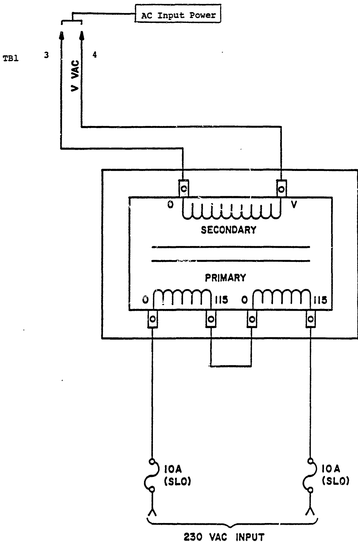
FIG. 4 240 VAC 50/60 HZ LINE INPUT 207
