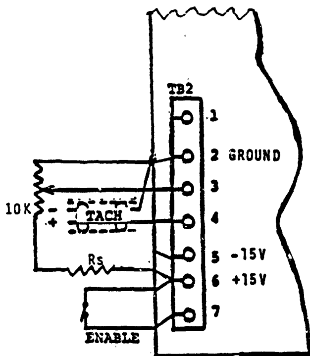
C. 1-direction control Tachometer Feedback
