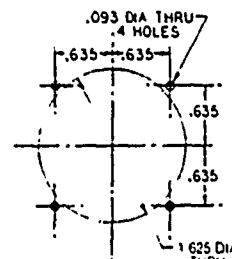
MOUNTING CUTOUT FOR ROUND BEZELS
