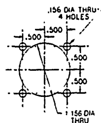
MOUNTING CUTOUT FOR SQUARE BEZELS
