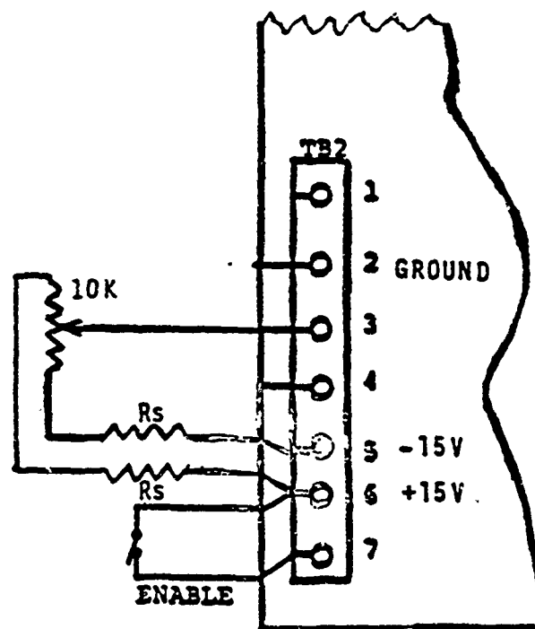
B. 2-direction control EMF Sensing
