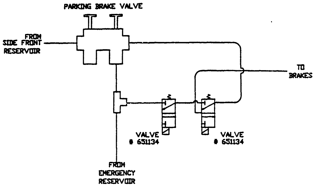
PARKING BRAKE
