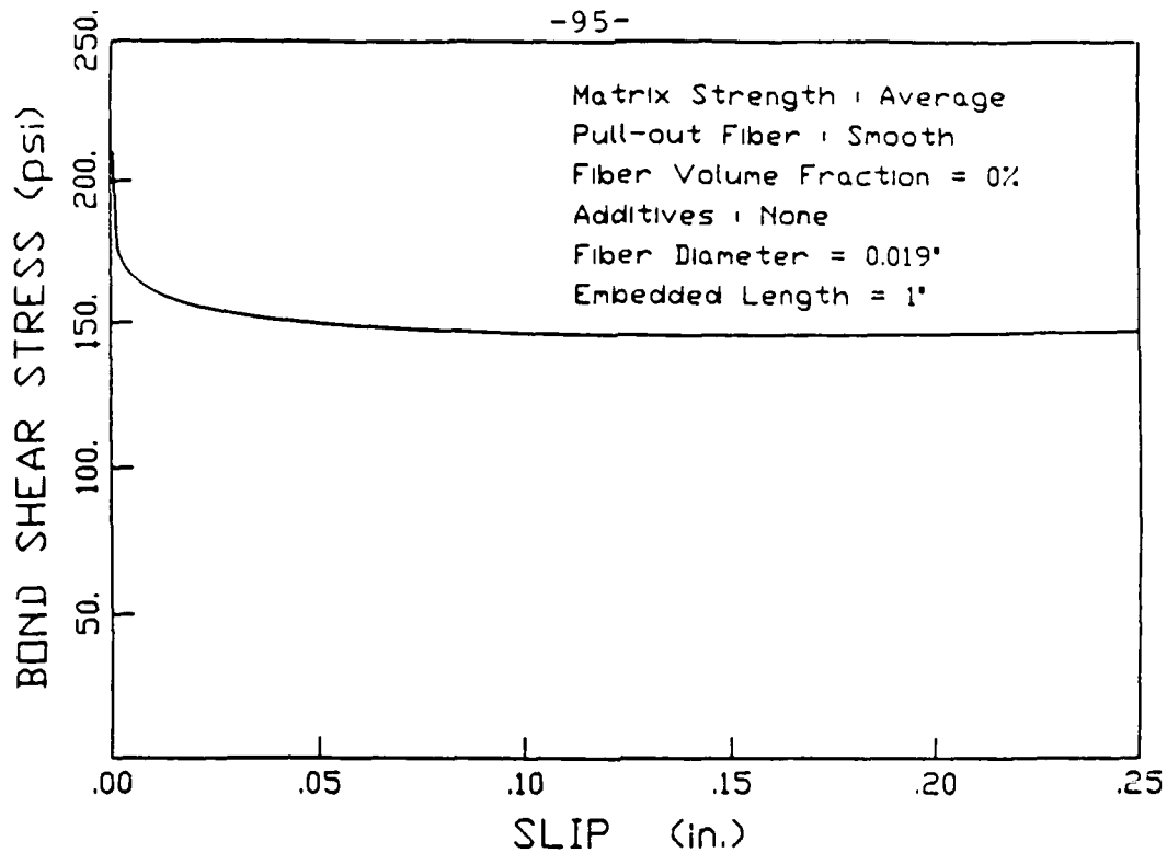
5.17a - Bond shear stress versus slip, A0SN series, full scale.
