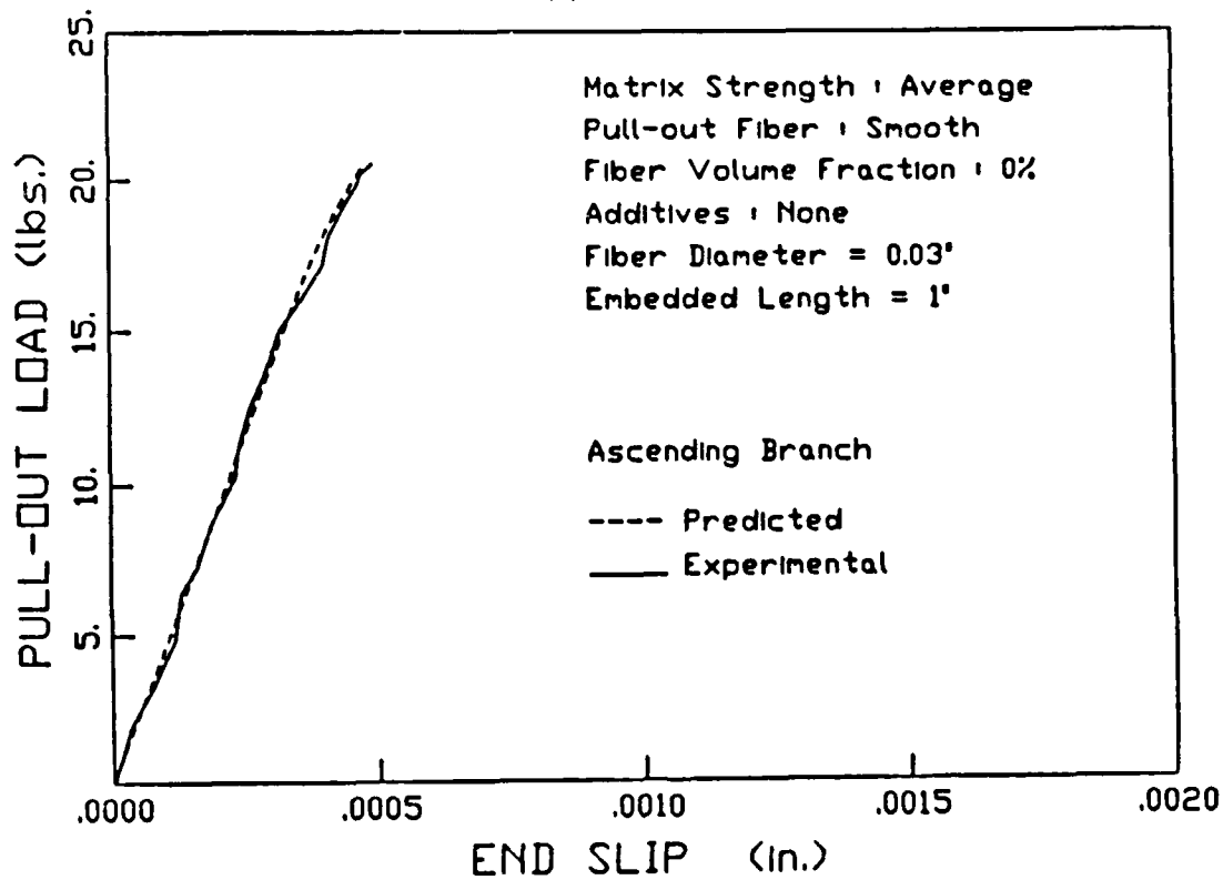
Fig. 6.28 - Experimental pull-out curve versus analytical prediction of pull-out curve of smooth fibers up to the peak load
