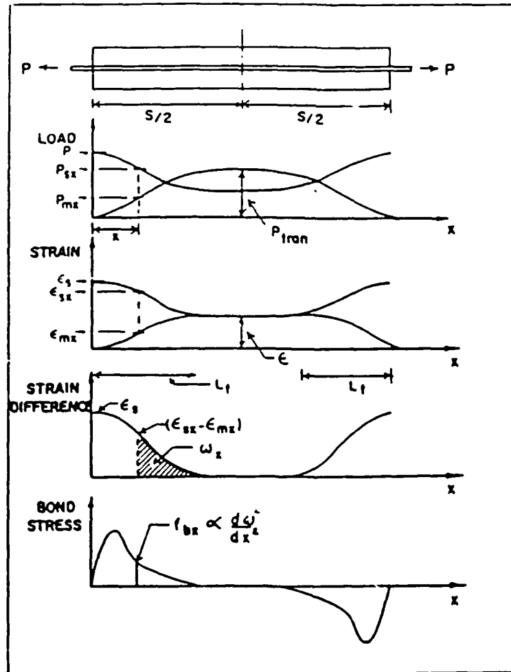
Fig. 3.4 - Load , strain, slip, and bond stress distribution (From Ref. 56).
