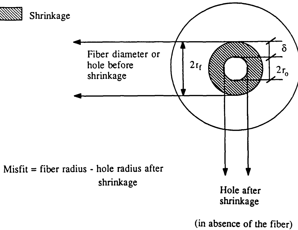
Fig. 5.9 - Fiber - matrix misfit
