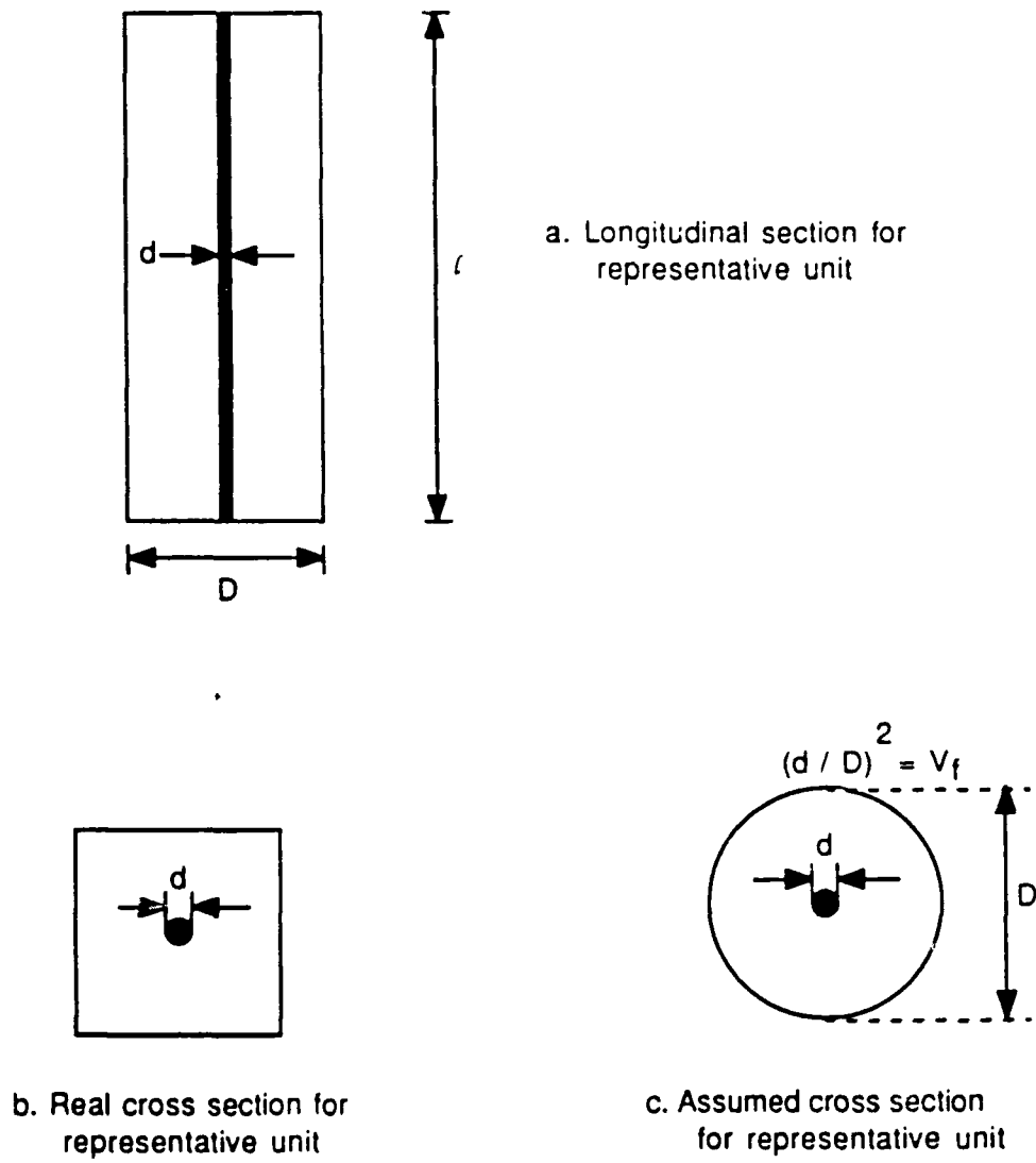
Fig. 7.3 - Typical representative unit.
