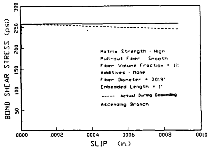
Bond shear stress versus slip, H1SN series, small scale.
