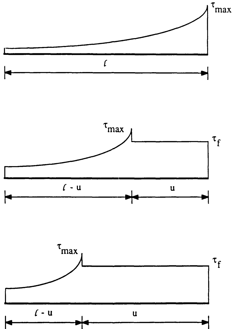
Fig. 5.4 - Typical bond stress distributions for cases where: (a) P = P_{\text{crit}} (b) P = P_1 > P_{\text{crit}} (c) P = P_2 > P_1 .
