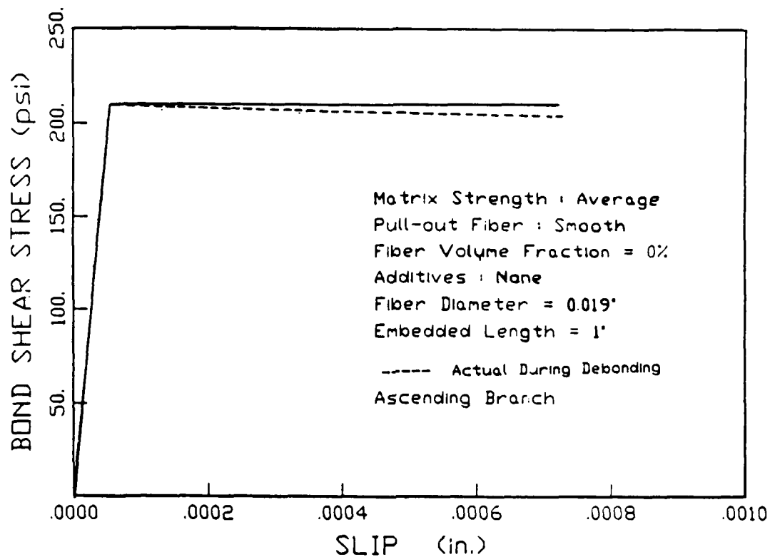
5.17b - Bond shear stress versus slip, A0SN series, small scale.
