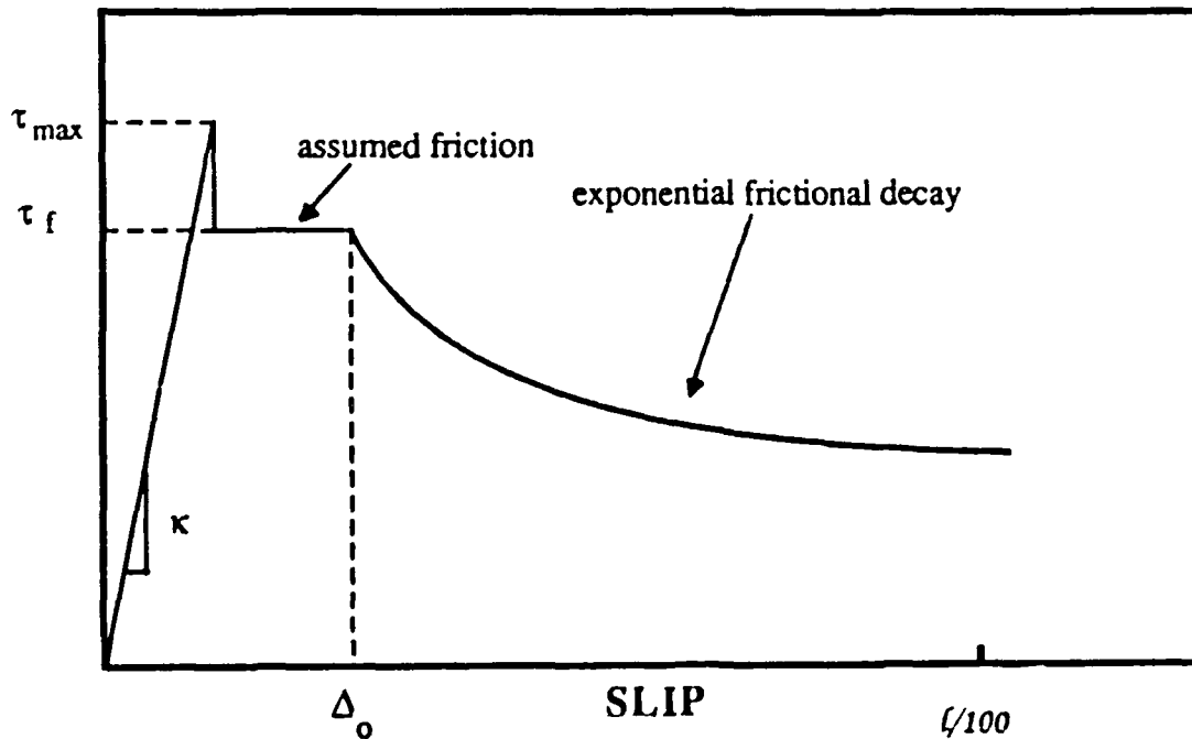
Fig. 5.8b - Alternative bond shear stress versus slip relationship with frictional decay when smaller scale.
