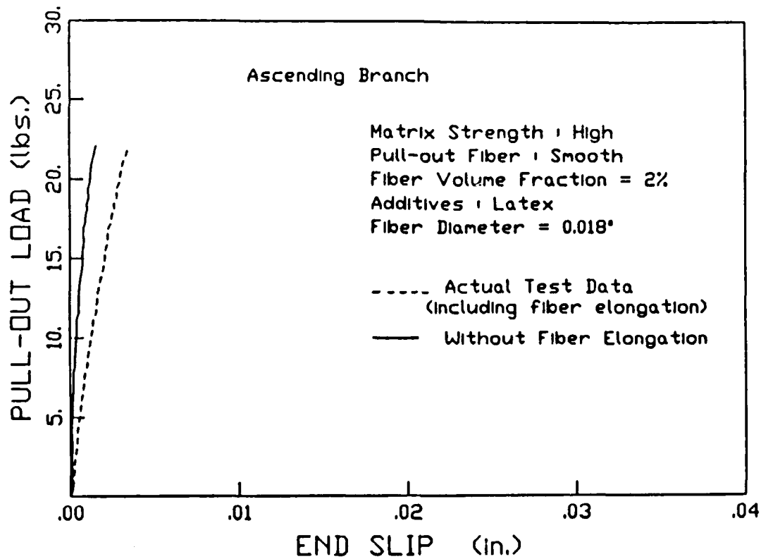
Fig. 6.8a - Typical pull-out load versus slip relationship of smooth fiber .
