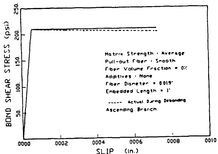
Bond shear stress versus slip, A0SN series, small scale.
