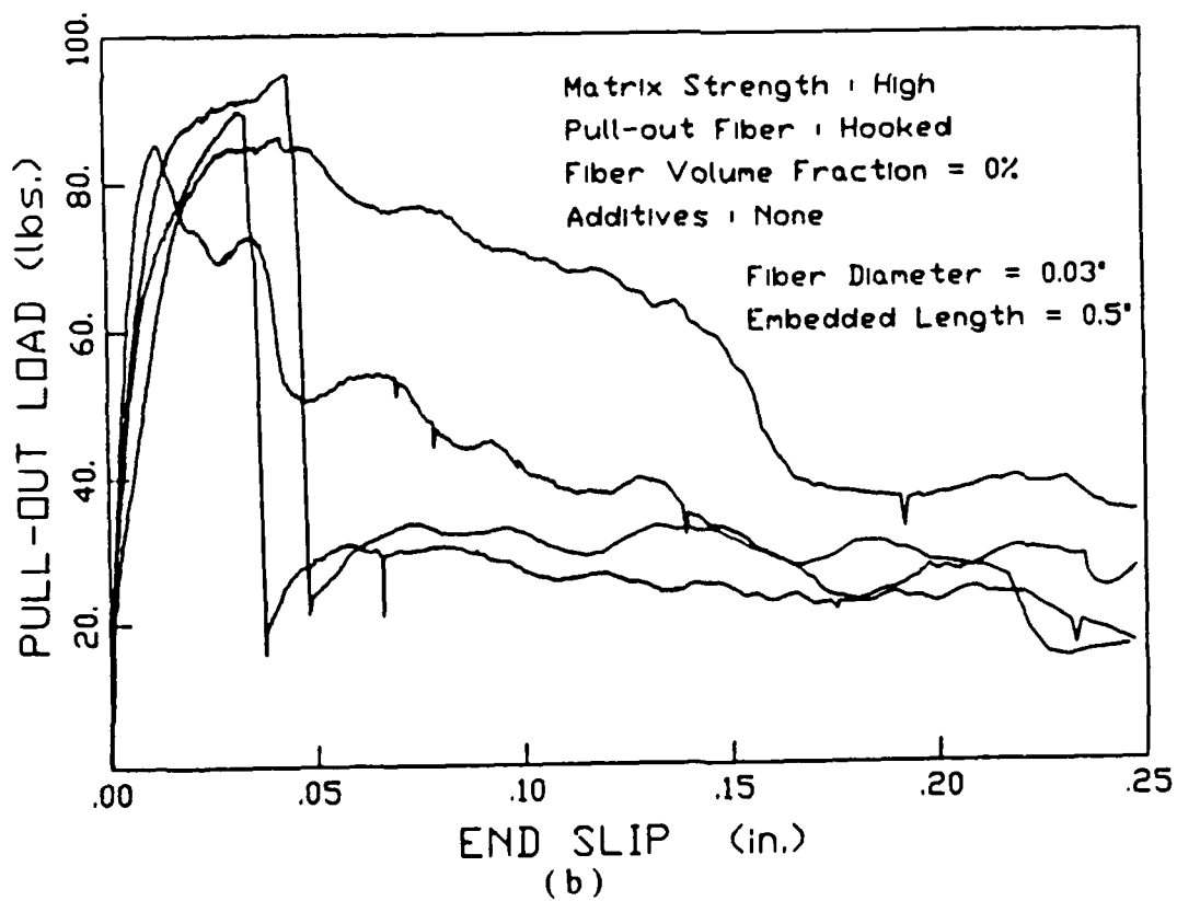
Fig. 6.21 - Pull-out load versus end slip of hooked fibers
