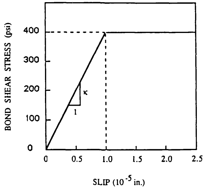
Fig. 7.6 - Assumed bond shear stress versus slip relationship in numerical example.
