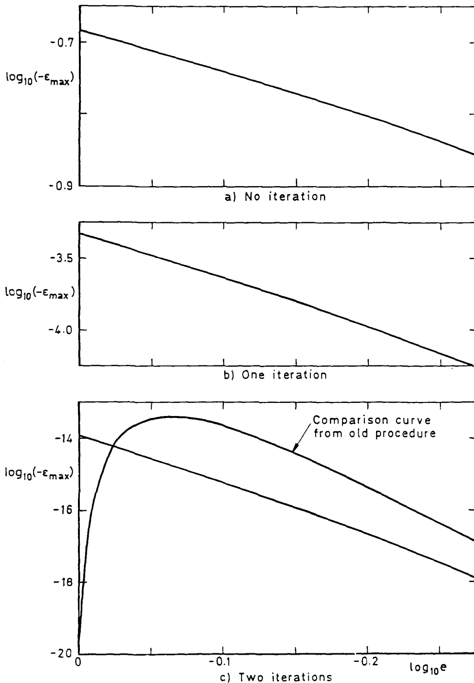
Fig 2 Maximum relative error (truncation) for the new solution procedure, EKEPL, for Kepler's classical equation
