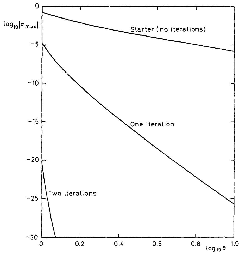
Fig 1 Maximum relative truncation error for the solution procedure, SHKEPL, for the reformulated hyperbolic equation ( \epsilon \leq 10 )
