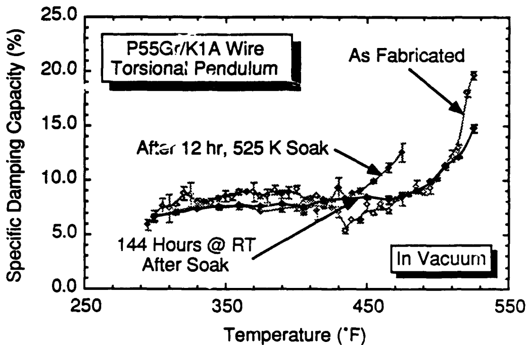
Figure 5.2.2.1-4 Thermal Dependence of the Damping in P55Gr/Mg-0.6%Zr (Gr/K1A) Precursor Wire After 144 Hours at Room Temperature: Indicating Most of the Initial Temperature Dependence of the Specimen Returning
