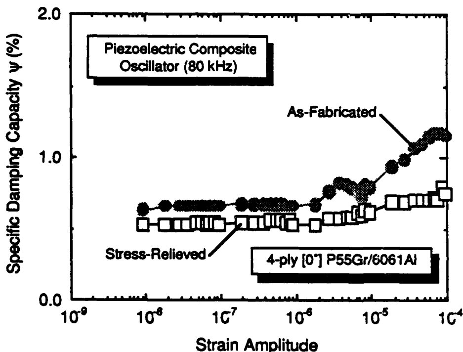
Figure 7.2-4 Damping Response of [0]_4 P55Gr/6061 Al by Piezoelectric Composite Oscillator Indicating a Lack of Strain Amplitude Dependence After Cryogenic Stress Relieving
