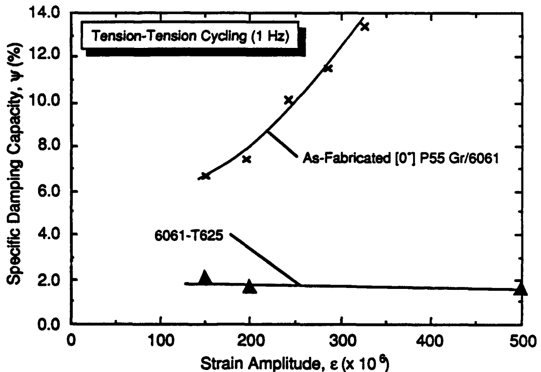
Figure 7.2-2 Damping Behavior of As-Fabricated [0°] P55/6061 Al Specimens in Tension-Tension Fatigue Tests Indicating Both Strain Amplitude Independent and Dependent Response and an Overall Greater Damping Capacity than Observed by Piezoelectric Composite Oscillator
