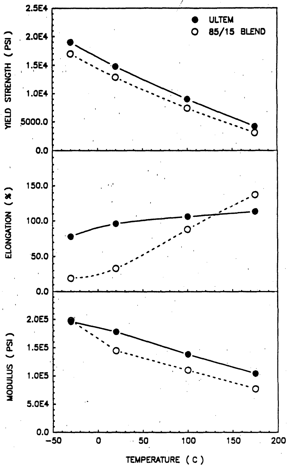
Figure 12: Yield Strength, Elongation, and Modulus of ULTEM and 85/15 ULTEM-VTOL BLEND AS A FUNCTION OF TEMPERATURE
