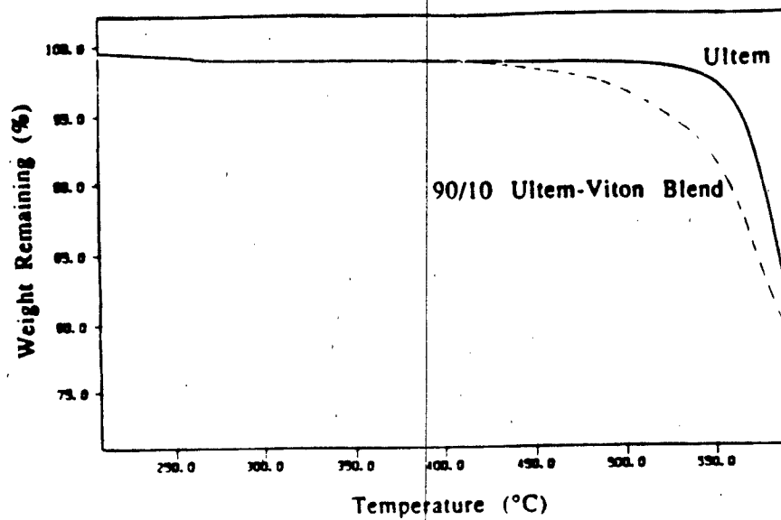
13 Figure 1: Thermogravimetric Analysis of Ultem and 90/10 Ultem-Viton Blend Produced by Compositional Quenching
