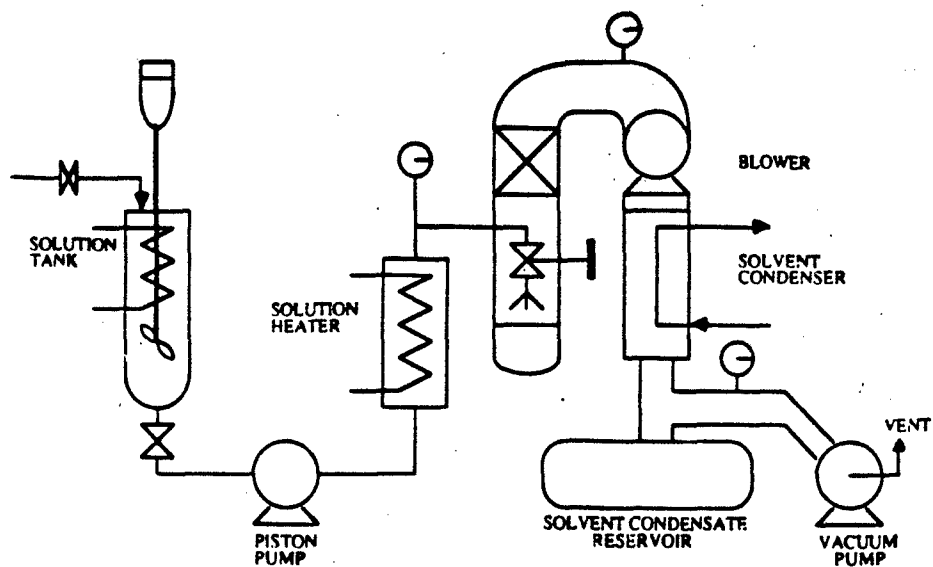
Figure 1: Schematic Diagram of Compositional Quenching Apparatus
