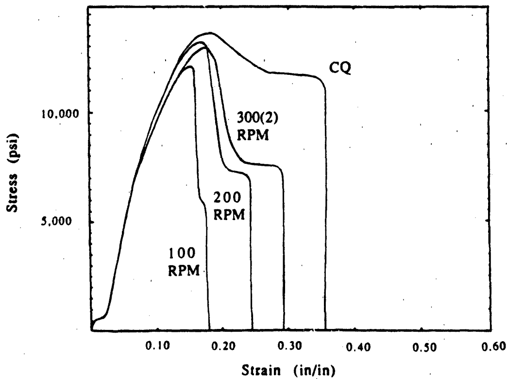
Figure 2: Tensile Test Stress - Strain Curves for 90/10 Ultem-Viton Blends
