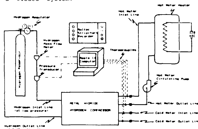
FIGURE 7 : Operational and Test Setup of the Hydride-Hydrogen Compressor
