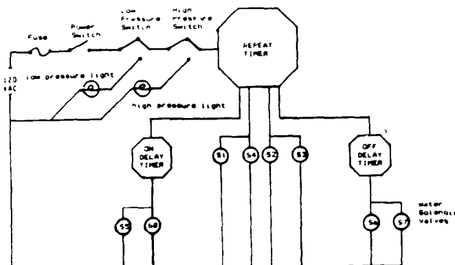
FIGURE 6 : Electrical Operational Schematic of Hydride-Hydrogen Compressor
