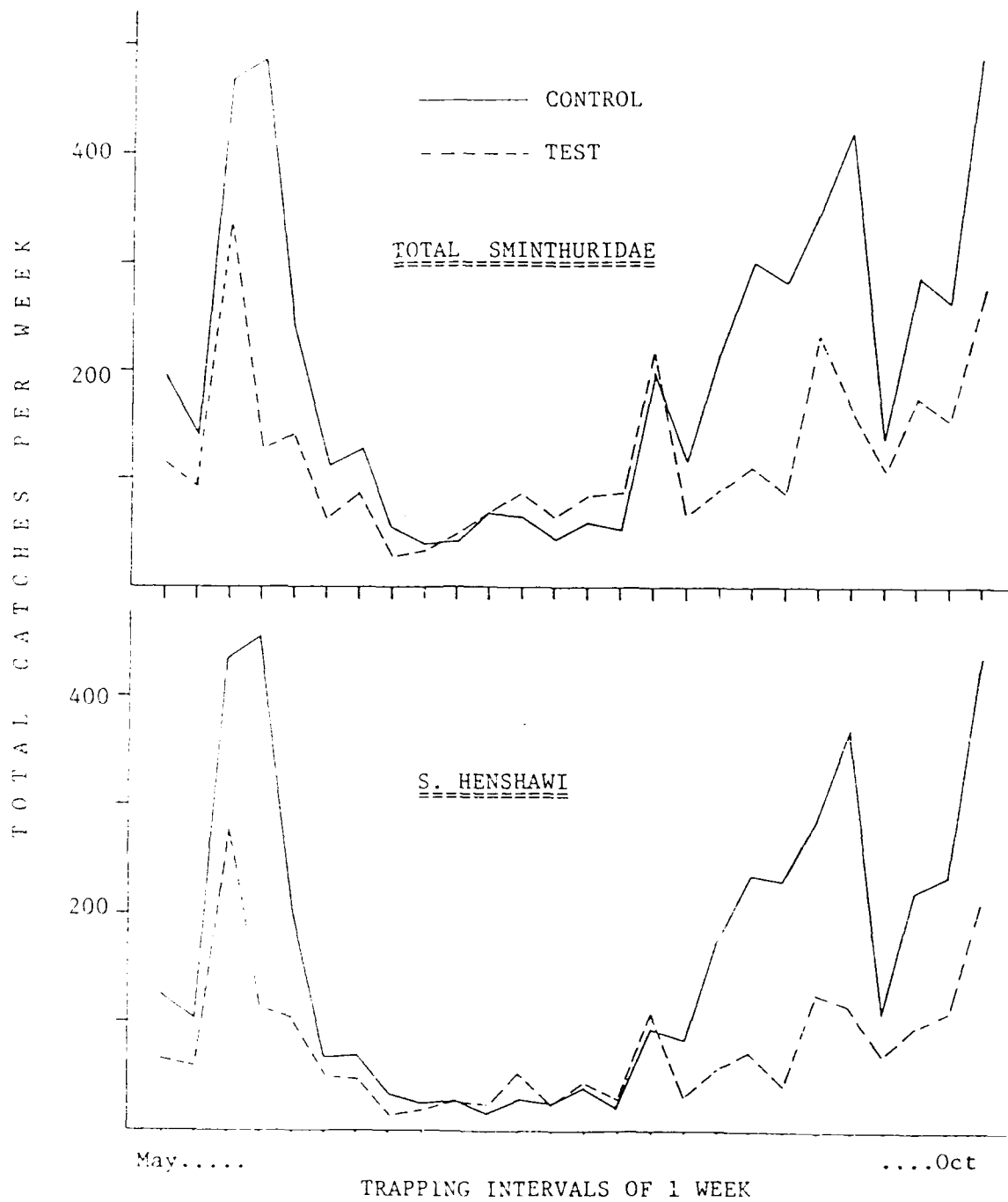
Fig. 17. Total catches, 1987, of total Sminthuridae and of S. henshawi in Test and Control. Dicyrtoma aurata and D. marmorata omitted from counts of sminthurids in Control.
