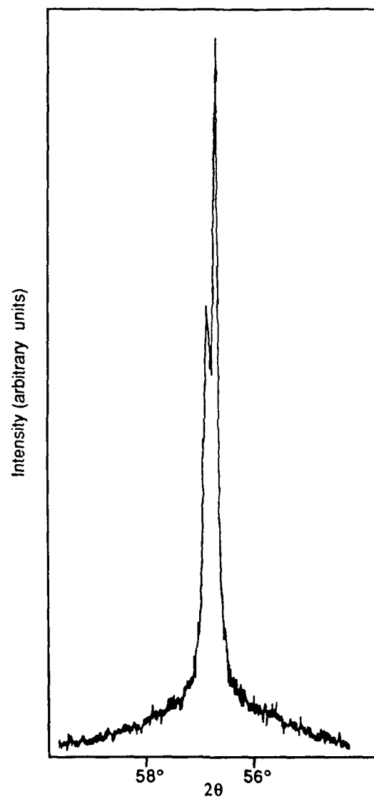
FIG. 5.33. X-RAY DIFFRACTION PEAKS FOR THE (400) REFLECTION FROM A 2.3 \mu\text{m} THICK CADMIUM TELLURIDE LAYER PHOTO-DEPOSITED ONTO A (100) GALLIUM ARSENIDE SUBSTRATE AT 300°C WITH DMCd:DETe=1 AND DEFOCUSSED UV.
