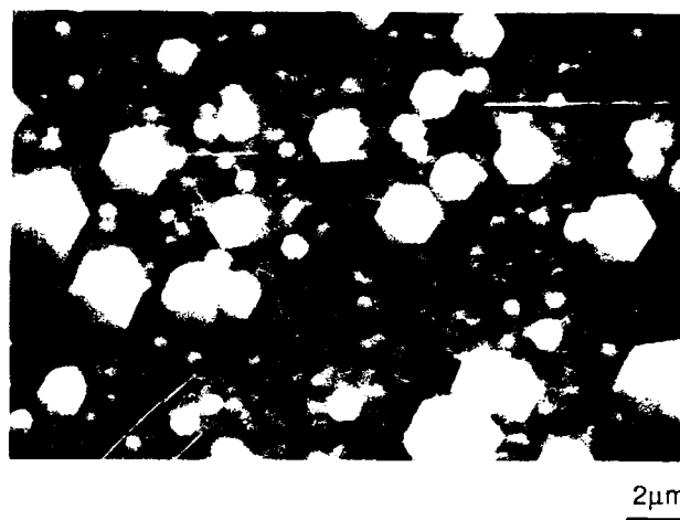
FIG 5.4. SURFACE MORPHOLOGY OF A CADMIUM TELLURIDE LAYER DEPOSITED ON A HYDROGEN CLEANED GALLIUM ARSENIDE SUBSTRATE AT 230°C WITH DET e RICH CONDITIONS AND FOCUSED UV.
