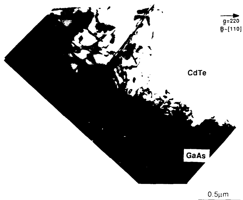
FIG. 5.6. GROSS-SECTIONAL TEM MICROGRAPH OF A CADMIUM TELLURIDE LAYER DEPOSITED ON A GALLIUM ARSENIDE SUBSTRATE AT 350°C WITH UNITY Z/ALRYL RATIO AND FOCUSSED UV
