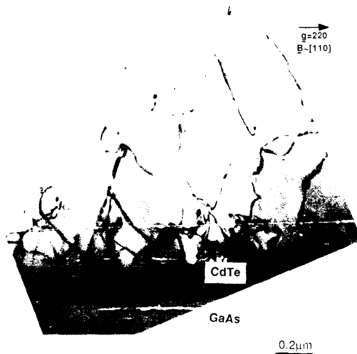
FIG. 5.22. CROSS-SECTIONAL TEM MICROGRAPH OF A CADMIUM TELLURIDE LAYER DEPOSITED THERMALLY ON A GALLIUM ARSENIDE SUBSTRATE AT 410°C WITH DMCd/DETe=0.81 .
