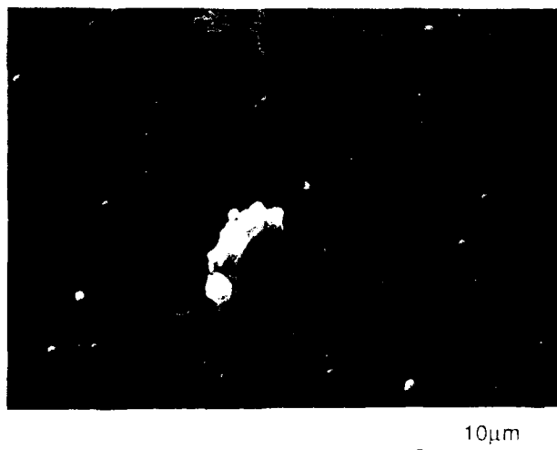
FIG. 6.5. SURFACE MORPHOLOGY OF CADMIUM DEPOSITED ON A SAPPHIRE SUBSTRATE (30 °C, 1.3 TORR PARTIAL PRESSURE, 1 HOUR)
