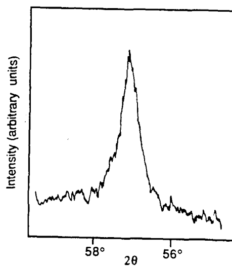
FIG. 5.35. X-RAY DIFFRACTION PEAK FOR THE (400) REFLECTION FROM A 0.3\mu\text{m} THICK CADMIUM TELLURIDE LAYER PHOTO-DEPOSITED ONTO A (100) GALLIUM ARSENIDE SUBSTRATE AT 250^{\circ}\text{C} WITH DMCD:DETE=2 AND DEFOCUSSED UV.
