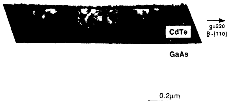
FIG. 5.27. CROSS-SECTIONAL TEM MICROGRAPH OF A CADMIUM TELLURIDE LAYER DEPOSITED THERMALLY ON A GALLIUM ARSENIDE SUBSTRATE AT 350°C WITH UNITY ALKYL RATIO.
