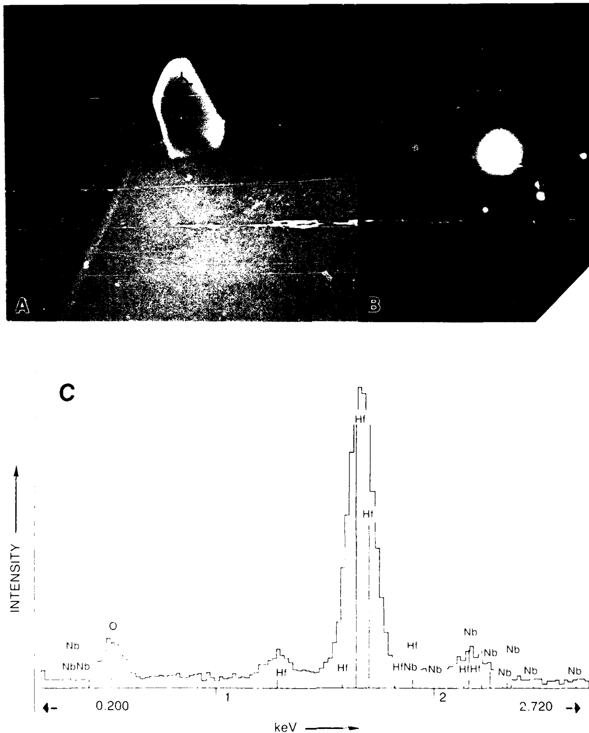
Figure 47. \text{HfO}_2 Grain Boundary Precipitate in Nb-0.6Hf-1.2N (at%), Aged at 1200^\circ\text{C}/4\text{h} + 1400^\circ\text{C}/8\text{h}
