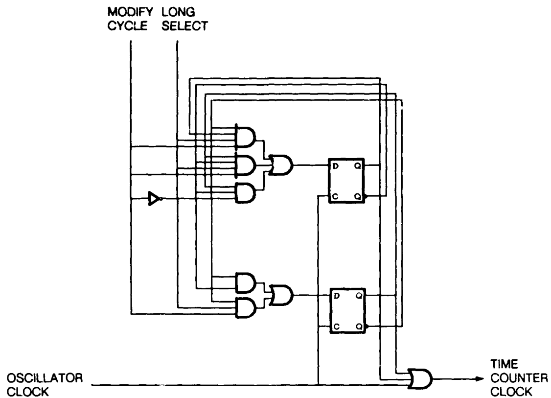
Figure 6. Divide-by-three phase counter implementation example.
