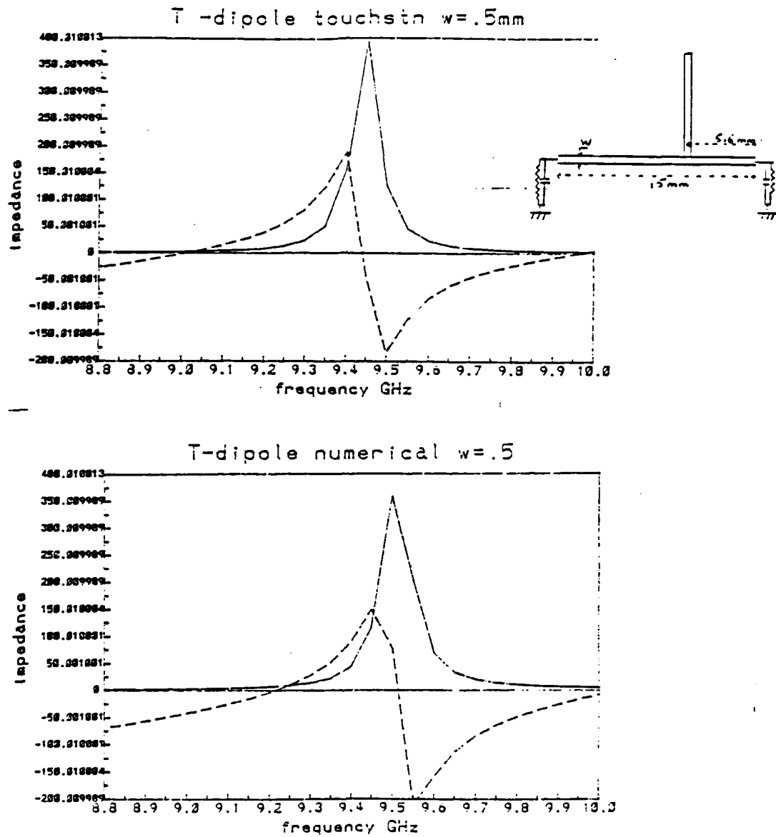
Figure 2 single dipole a -computation by Touchstone b - Moment method w=.5\text{mm} h=1.\text{mm} \epsilon_r=1.0
