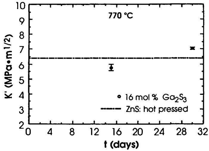
FIG. 6 Variation of the "effective" fracture toughness, K' , as a function of transformation time, t , at 770 °C for the 16 mol % alloy of 99.0 % theoretical density.
