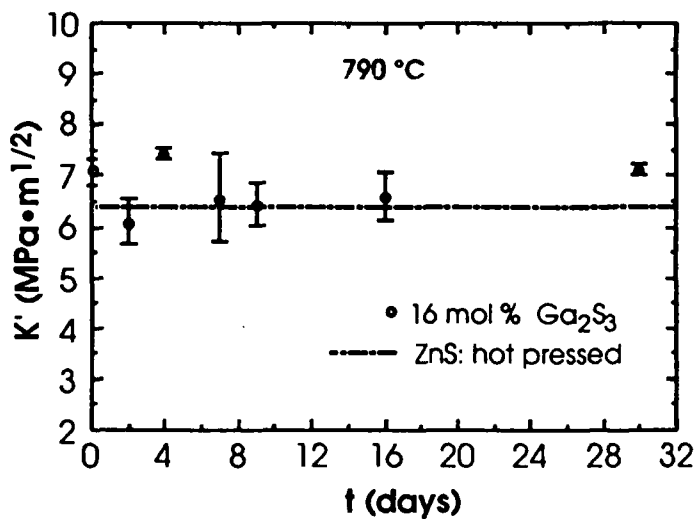
FIG. 5 Variation of the "effective" fracture toughness, K' , as a function of transformation time, t , at 790\text{ }^{\circ}\text{C} for the 16 mol % alloy of 97.4 % theoretical density.
