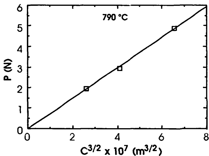
FIG. 4 Indentation load, P , vs the 3/2 power of the crack length, C , for the 16 mol % alloy transformed at 790\text{ }^{\circ}\text{C} for 4 days.
