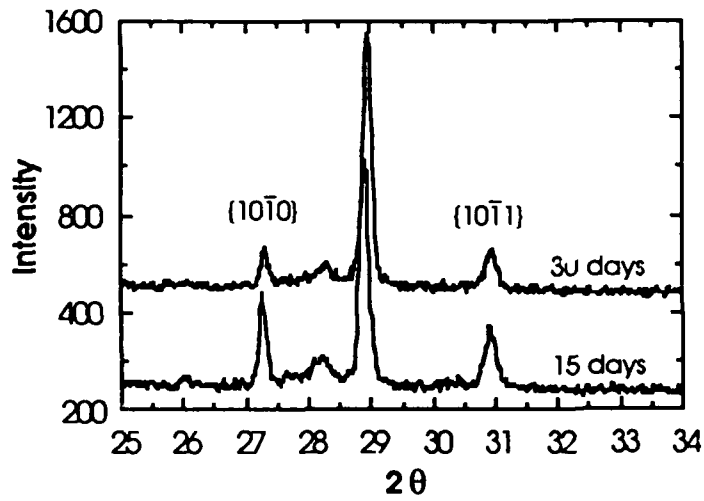
FIG. 7 Comparison of the intensities of the (10\bar{1}0) and (10\bar{1}1) wurtzite peaks in the 99.0 % dense sample after transformation times of 15 and 30 days at 770 °C.
