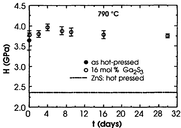
FIG. 3 Vickers hardness, H , as a function of transformation time, t , at 790\text{ }^{\circ}\text{C} for the 16 mol % alloy of 97.4 % theoretical density.
