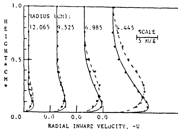
Fig. 3 Predicted and Measured Radial Velocity on Solid Surface. (Keys: o & —, Measured & Calculated values on Smooth Surface; o & ---, Measured & Calculated values on Rough Surface of Sand Grain Mesh #120)
