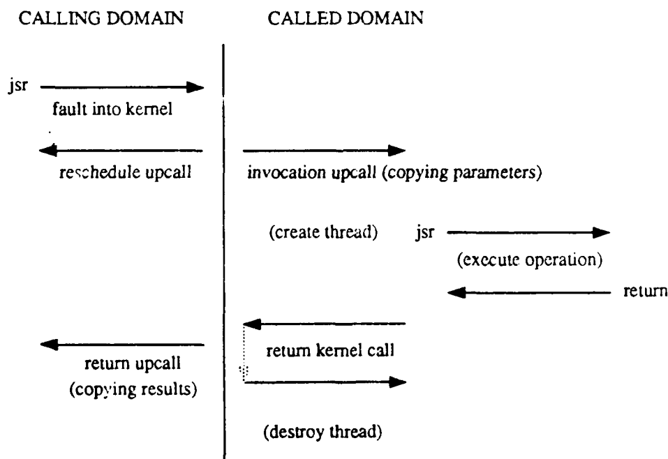
Figure 3: Protected Invocation
