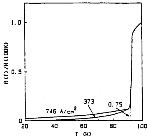
Figure 4. The superconducting transition of a normally-sintered sample of \text{YBa}_2\text{Cu}_3\text{O}_7 at various current densities. The sample resistance at 100K is 6\text{m}\Omega .
