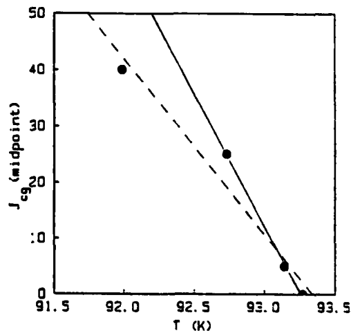
Figure 8. The intrinsic critical current density, J_{cg} , of the individual grains, versus absolute temperature for an under-sintered sample of \text{YBa}_2\text{Cu}_3\text{O}_7 . Two different linear extrapolations give J_{cg}(77\text{K}) values of 2 \times 10^4\text{ A}/\text{cm}^2 (dashed line) and 3 \times 10^4\text{ A}/\text{cm}^2 (solid line).
