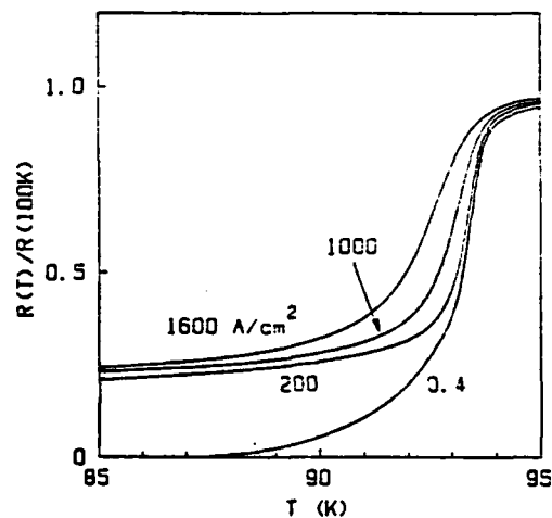
Figure 7. The main superconducting transition of an under-sintered sample of \text{YBa}_2\text{Cu}_3\text{O}_7 at various current densities. The temperature scale has been greatly expanded to show the shift in the transition midpoint.
