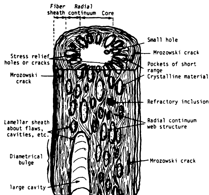
Figure 16. The Holey Curved Bundles of Graphite Sheets Model of Carbon Fiber Morphology of Barnet and Noor [6,7].
