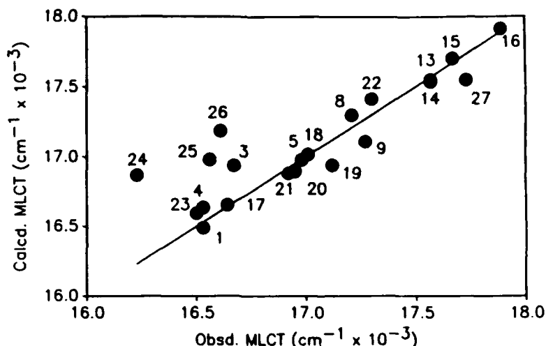
Fig. 7. Calculated versus observed \lambda_{\text{max}} for \text{Ru}(\text{DTBSq})_3 . Energies are calculated from equation 4. Solvents are numbered as in Table 1, with 17 = dimethylformamide, 18 = methanol, 19 = ethanol, 20 = 1-propanol, 21 = 1-butanol, 22 = toluene, 23 = 1,2-dichlorobenzene, 24 = 1,2-dichloroethane, 25 = dichloromethane, 26 = trichloromethane, 27 = tetrachloromethane.
