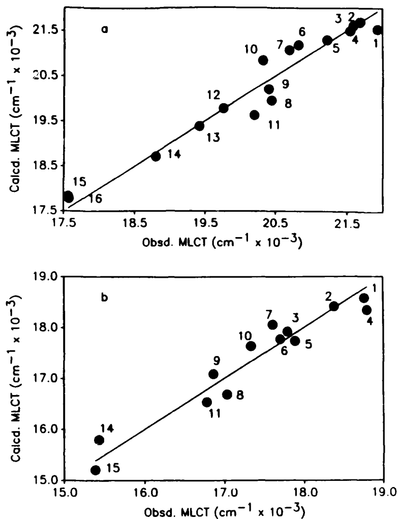
Fig. 4. Calculated versus observed transition energies for MLCT 1: (a) \text{Mo(CO)}_4\text{bpm} , (b) [\text{Mo(CO)}_4]_2\text{bpm} . Energies are calculated from equation 1 using parameters in Table 2. Solvents are numbered as in Table 1.
