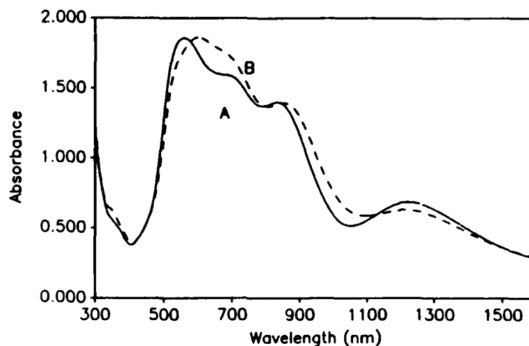
Fig. 8. Electronic spectra of 1.5 \times 10^{-4} M \text{Ru}(\text{DTBSq})_3 in hexane — (A) and acetonitrile --- (B).
