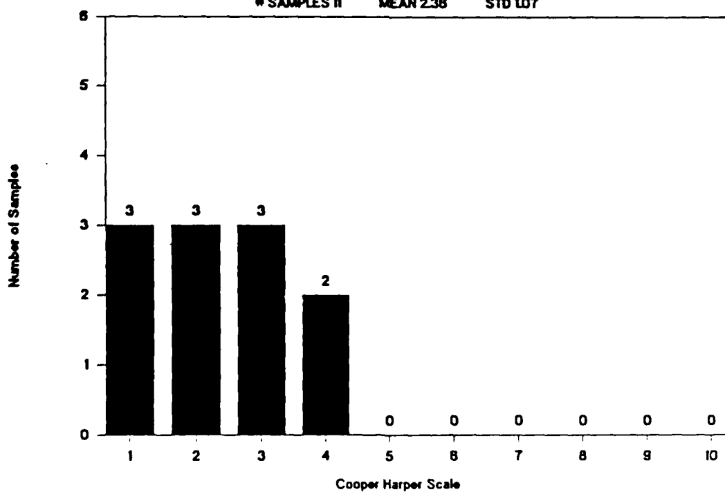
FIGURE 9. DECELERATION RATING HISTOGRAM OF PILOT RESPONSE (SHEET 2 OF 2)
