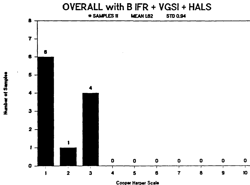
FIGURE 5. OVERALL RATING HISTOGRAM OF PILOT RESPONSE (SHEET 2 OF 2)
