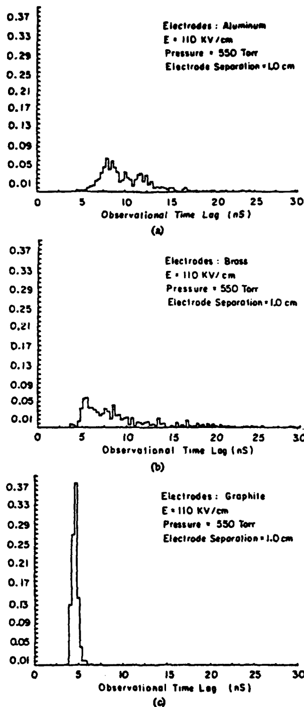
Figure 2. Observational time lag for three different electrode materials as determined by Levinson and Kunhardt [1982].
