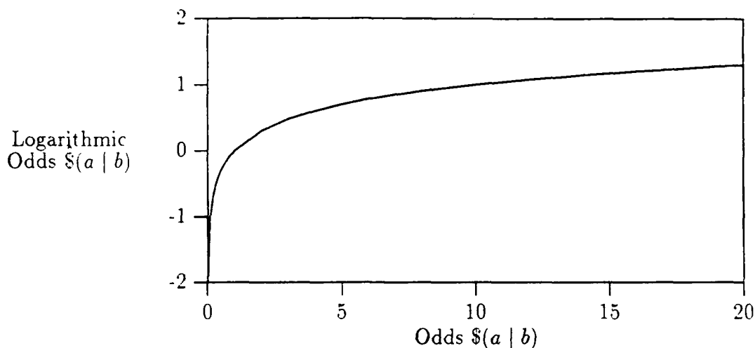
Figure 6.1: Odds values vs. logarithmic odds values. A log odds ratio of zero means equal weight to a fluent and its negation. a positive value means more weight to the unnegated fluent, and a negative value means more weight to the negated fluent.
