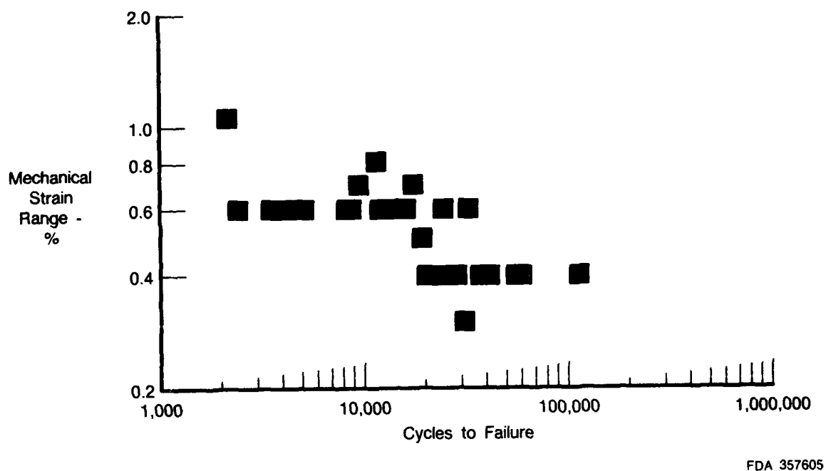
Figure 35. Mechanical Strain Range Versus Fatigue Life for All Uncoated PWA 1480 TMF Tests
