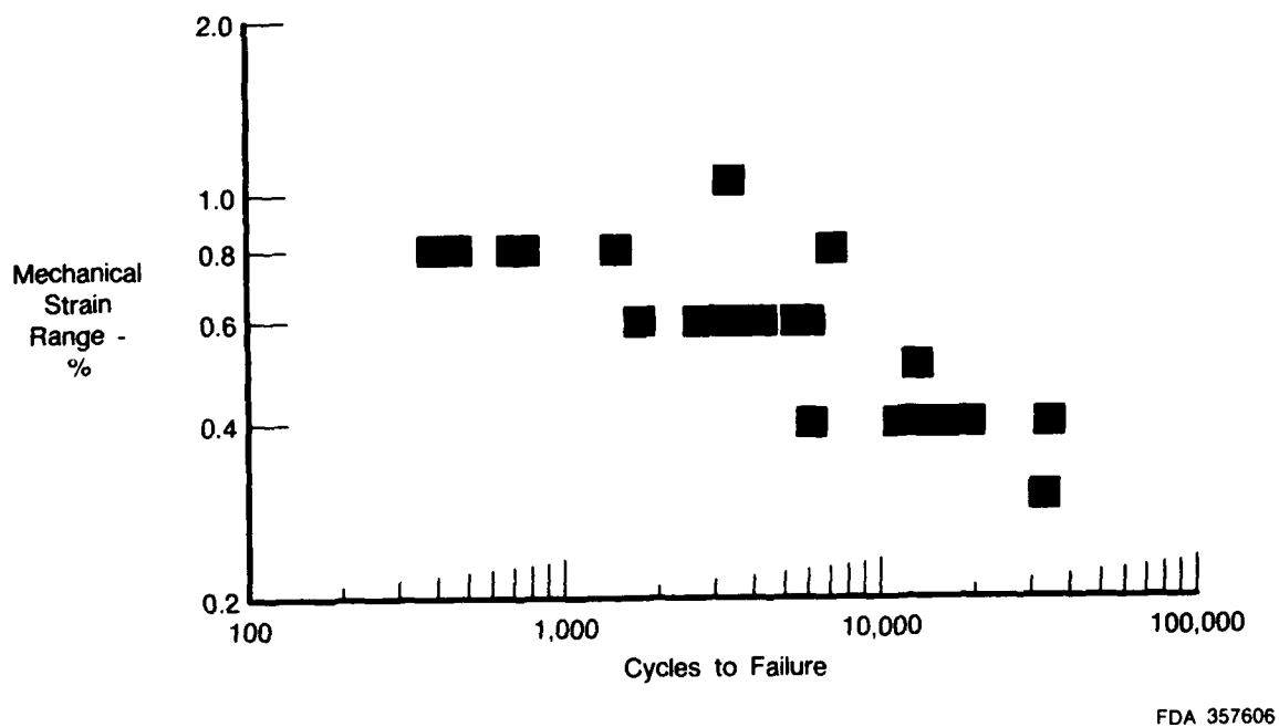
Figure 36. Mechanical Strain Range Versus Fatigue Life for All PWA 275 Coated PWA 1480 TMF Tests
