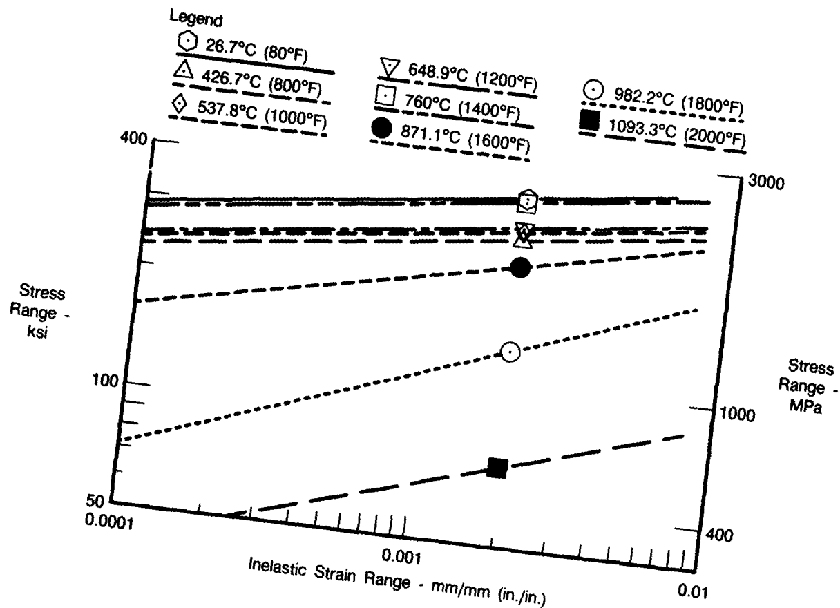
Figure 31. Inelastic Strain Versus Stress Range for PWA 1480 (0.2% Inelastic Strain)
