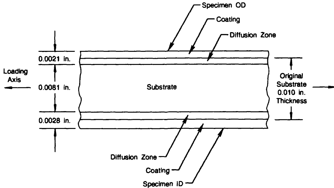
Figure 22. Post Test Measurement of Substrate and Coating Thickness
