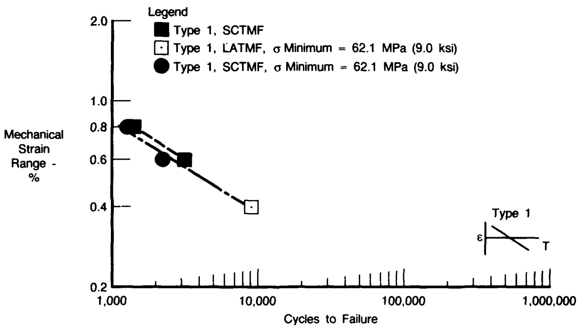
Figure 45. Controlled Minimum Stress Effects on PWA 286 Coated PWA 1480 (Out-of-Phase TMF Cycle, 1 cpm, 427-1038°C (800-1900°F))
