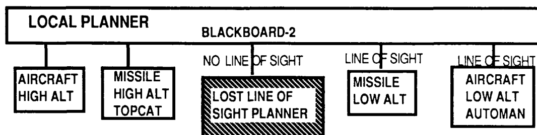
Figure 2: Extended REACT Architecture
