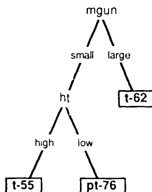
Figure 1. One procedural form for identifying Soviet tanks on the battlefield.
