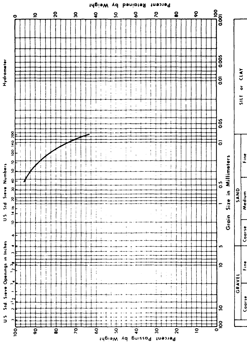
Figure D-18: GRAIN SIZE DISTRIBUTION; CYCLIC TRIAXIAL TEST NO. 21
