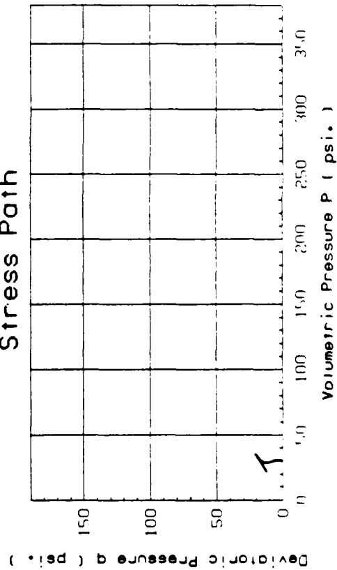
Figure A-8: IC-U TRIAXIAL TEST NO. BS3-8
