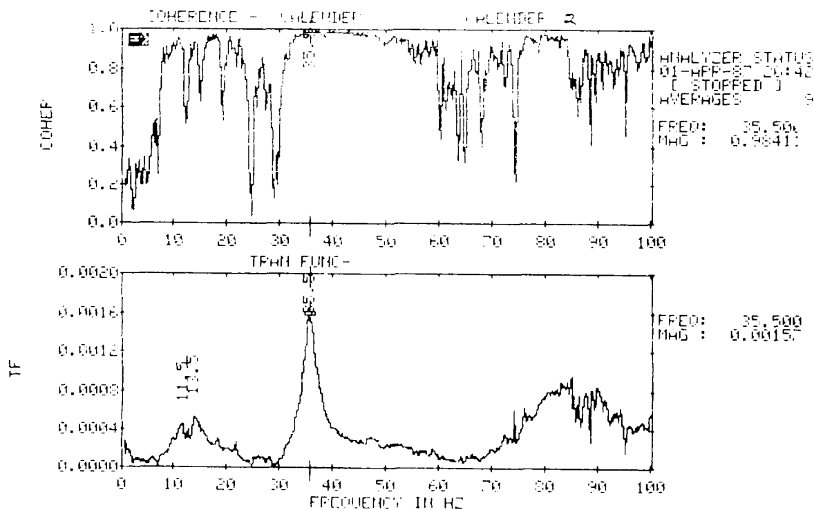
Figure 4. Transfer function (mobility) and coherence records for calendar impact test
