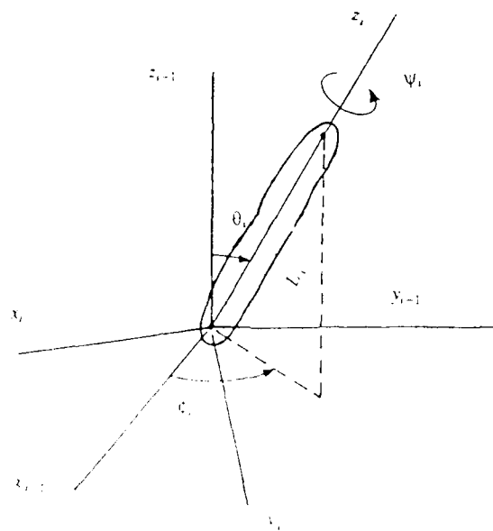
Figure 1. n Bar Linkage System
