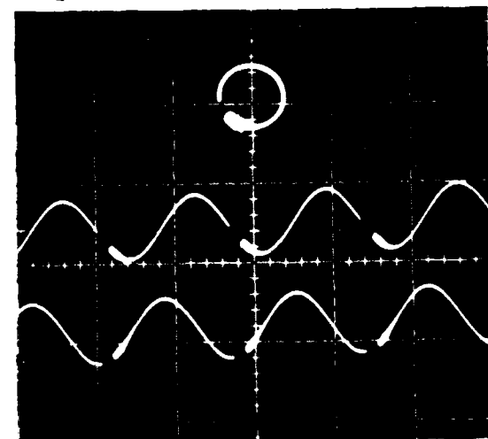
Fig.16b:Shaft-B Orbit/Time
