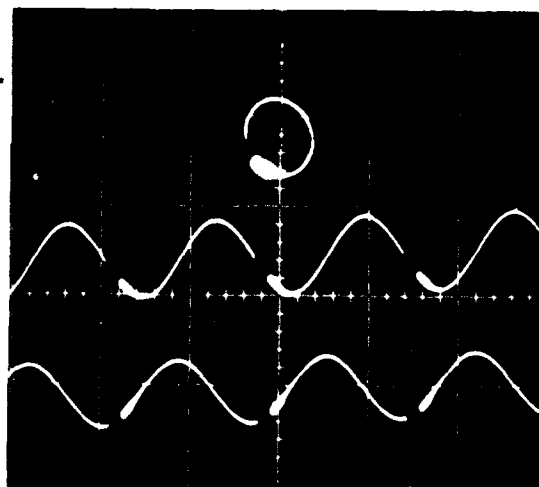
Fig.12b:Shaft-B Orbit/Time
