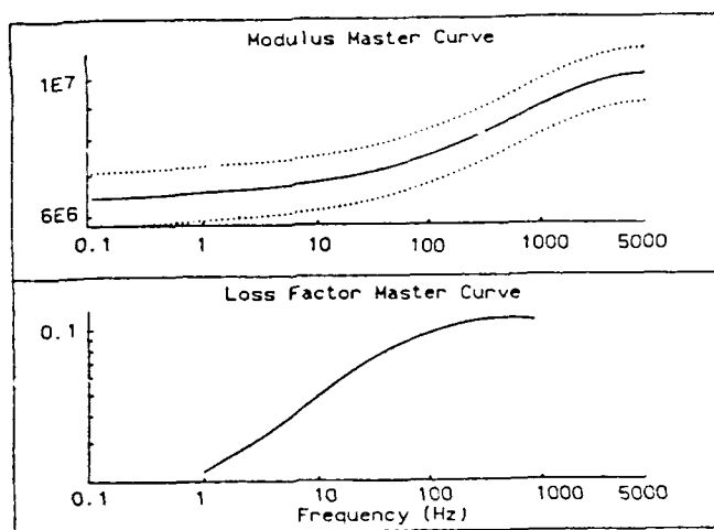
Figure 15 Assumed complex modulus master curves
