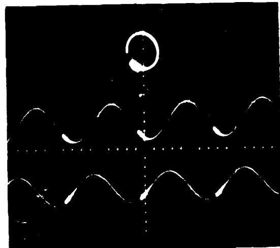
Fig.15b:Shaft-B Orbit/Time
