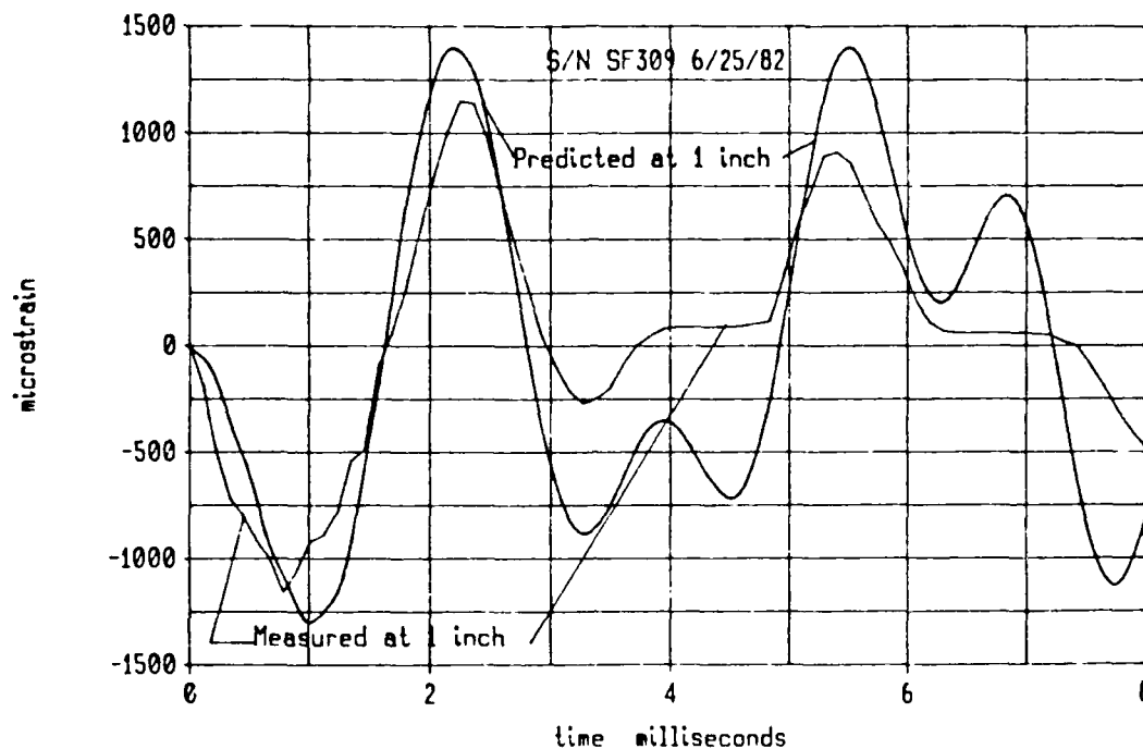
Figure 8 - Measured & Predicted Strain vs Time due to Ballotting
