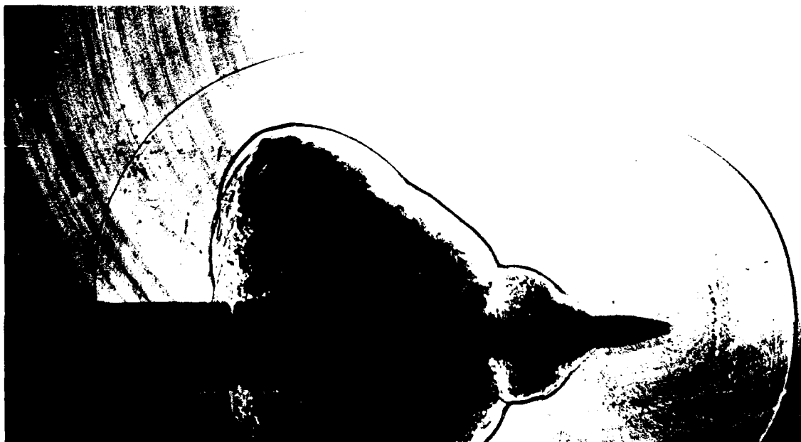
Fig. 11 Pressure contour plot and shadowgraph for the brake case, t = 0.423 \text{ msec.}
