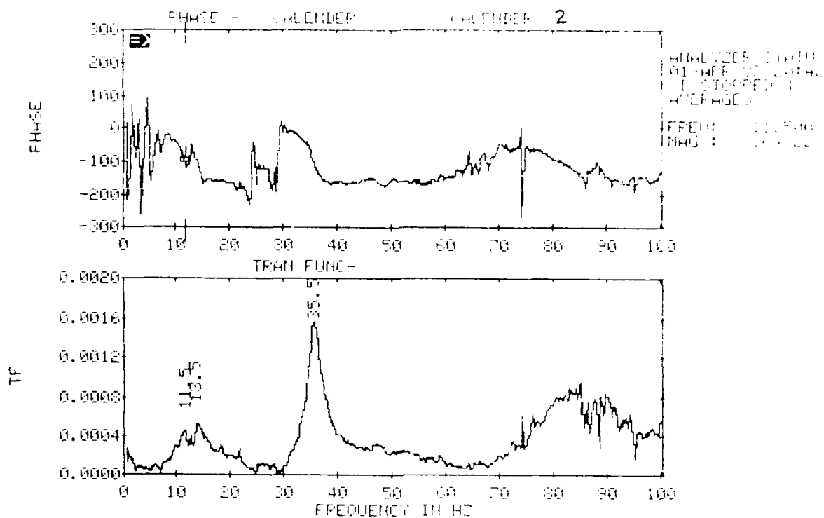
Figure 3. Transfer function (mobility) and phase records for calendar impact test
