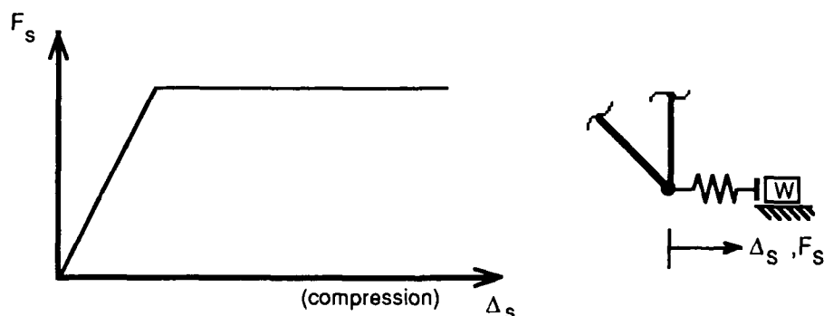
Figure 5. Elasto-plastic one-way soil support spring.
