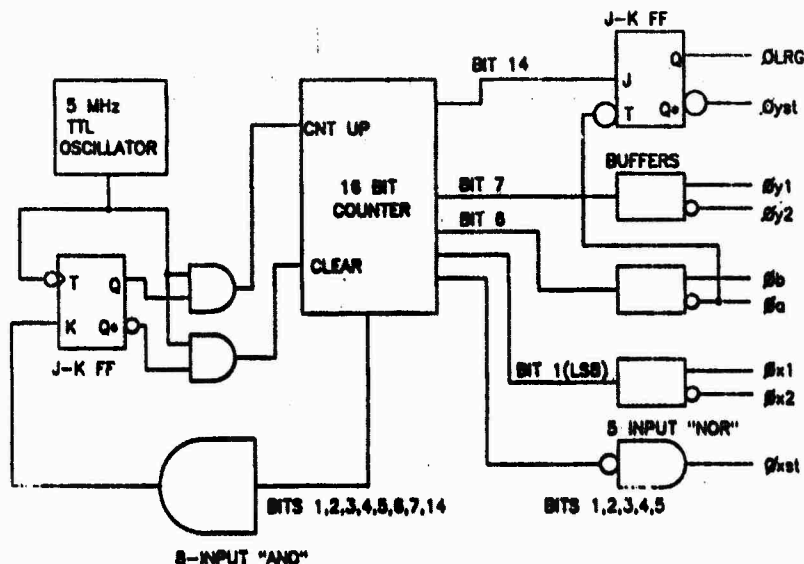
Figure 13. Scan Clock Generation Logic
