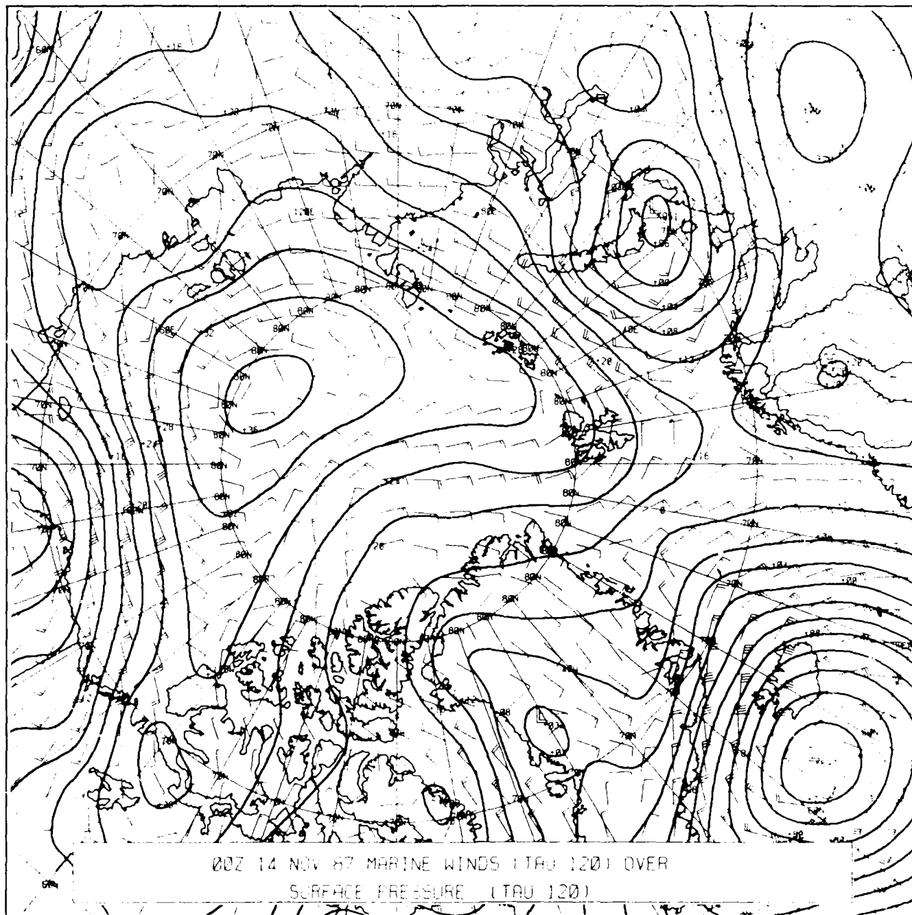
Figure 21b. Tau 120 NOGAPS surface pressures from the 14 November 1987 run.
