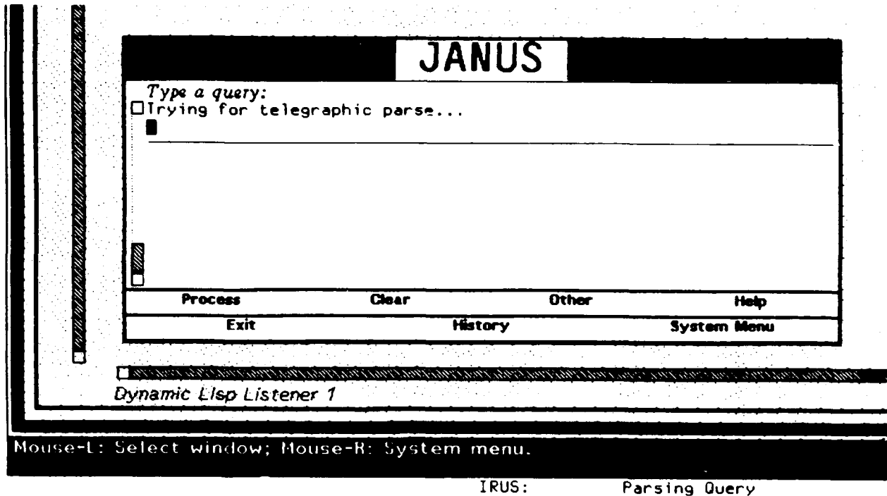
Figure 5: Message to end-user
