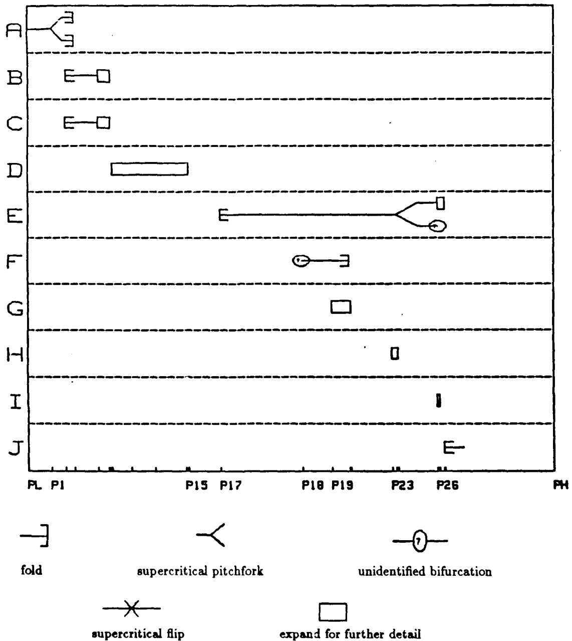
Figure 1: This diagram, generated automatically by the Bifurcation Interpreter, shows the analysis of the system described by equation (1) for k = 0.1 . The Interpreter has traced the evolution of 10 classes of families of periodic orbits and their bifurcations. Each bifurcation type is identified by a standard symbol—the key indicates the Interpreter's symbols for fold bifurcations, supercritical-pitchfork bifurcations, and for bifurcations that the Interpreter has failed to identify. The blank rectangles indicate parameter intervals over which the figure should be expanded to reveal more detail, as shown in figures 2 and 3. The p values along the horizontal axis indicate the parameter values at which the bifurcations occur.
