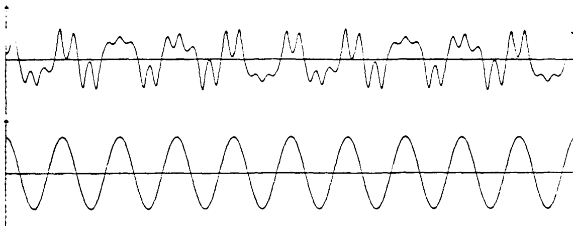
Figure 5: Shown here and in figure 6 are classes of steady-state orbits automatically reported by the Bifurcation Interpreter for the system in equation (1) that are missing from a well-known published catalogue of orbits for this system [20]. Plotted here are x(t) and the drive for an order-5 orbit from class J of figure 1 ( k = 0.1, p = 24.25 ).
