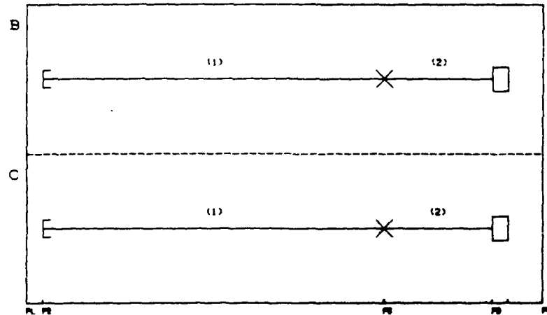
Figure 2: Expanding the interval from p = 3 to p = 5.7 shows details of classes B and C from figure 1. Each class begins as order 1, then doubles to order 2 via supercritical-flip bifurcations. Expanding the interval indicated by the rectangles would show further doubling. The Interpreter recognizes this progression as a period-doubling cascade, and reports it as such.
