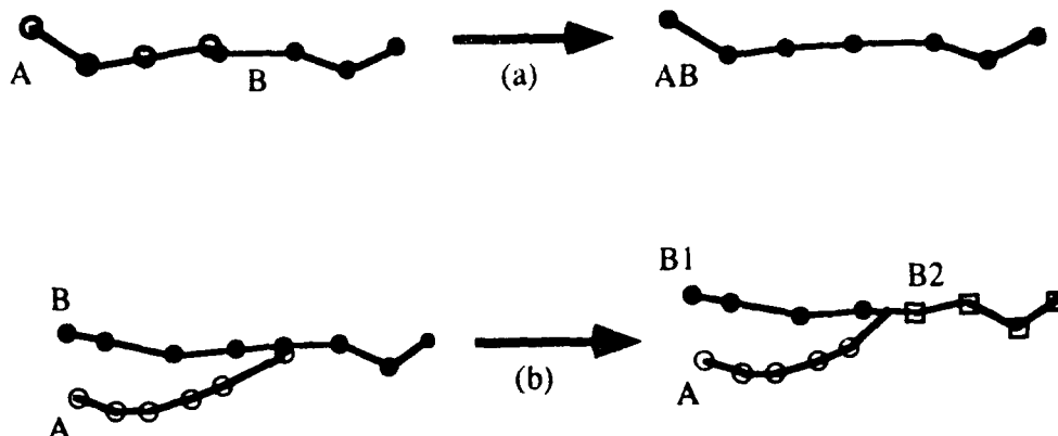
Figure 10: Merging families: (a) If family A extends to meet the first known instance of B , the two families are merged to form a single family AB . (b) If A coincides with a point in the middle of B (at a synchronization value of the parameter), B is split into two families B_1 and B_2 . A and B_1 vanish together at a bifurcation somewhere before the synchronization point, and B_2 appears there. Note that, in this figure, the horizontal direction represents the p -axis, while the vertical direction represents the location of the points in state space (projected onto a one-dimensional subset).
