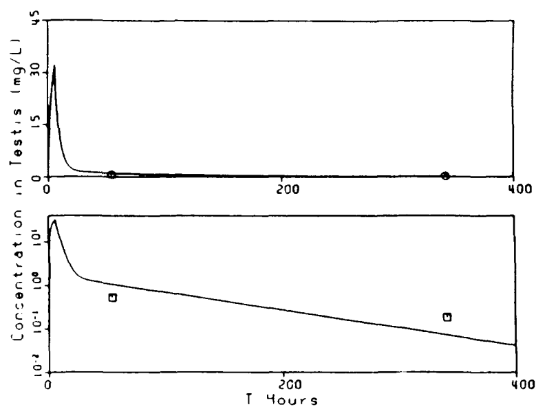
Figure 20. Concentration of CTFE (Group I Oligomers) in testes during and after single 0.5 mg/L, 6-h exposure. Solid lines represent simulations, points represent data. Linear plot, upper curve and hexagonal points. Log plot, lower curve and square points.
