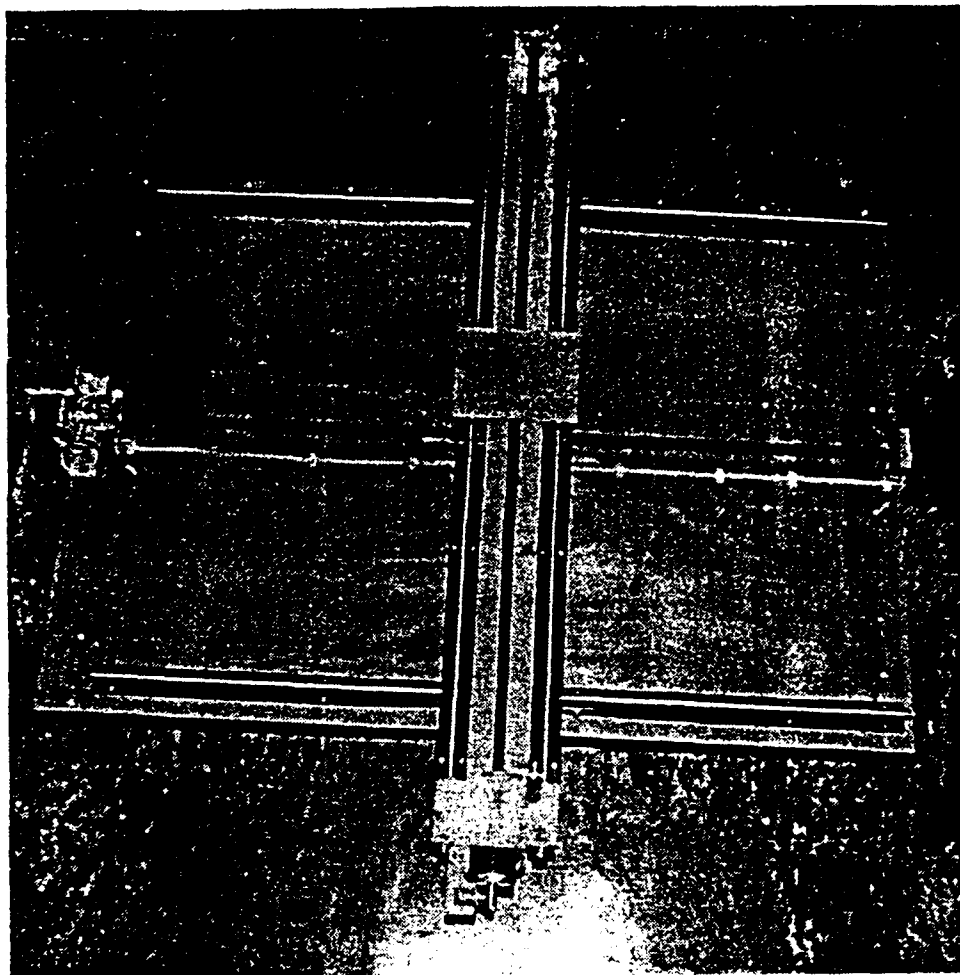
FIGURE 3. PROBE CARRIAGE
