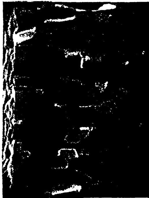
PURE Mo - ANNEALED AT 1000°C FOR 8 hr
