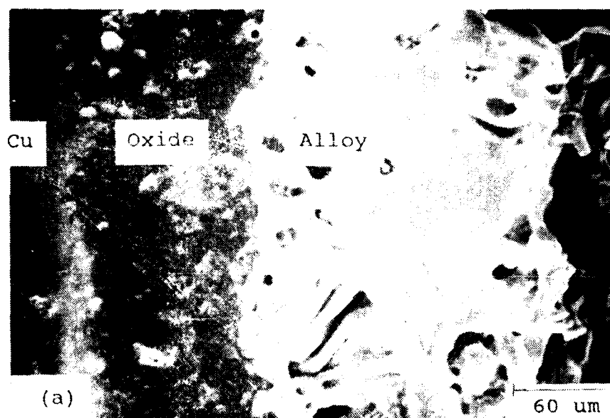
Fig. 23. Mo-40 Al-30 Si 1 atm Oxygen 800 Hours T= 1,550°C
