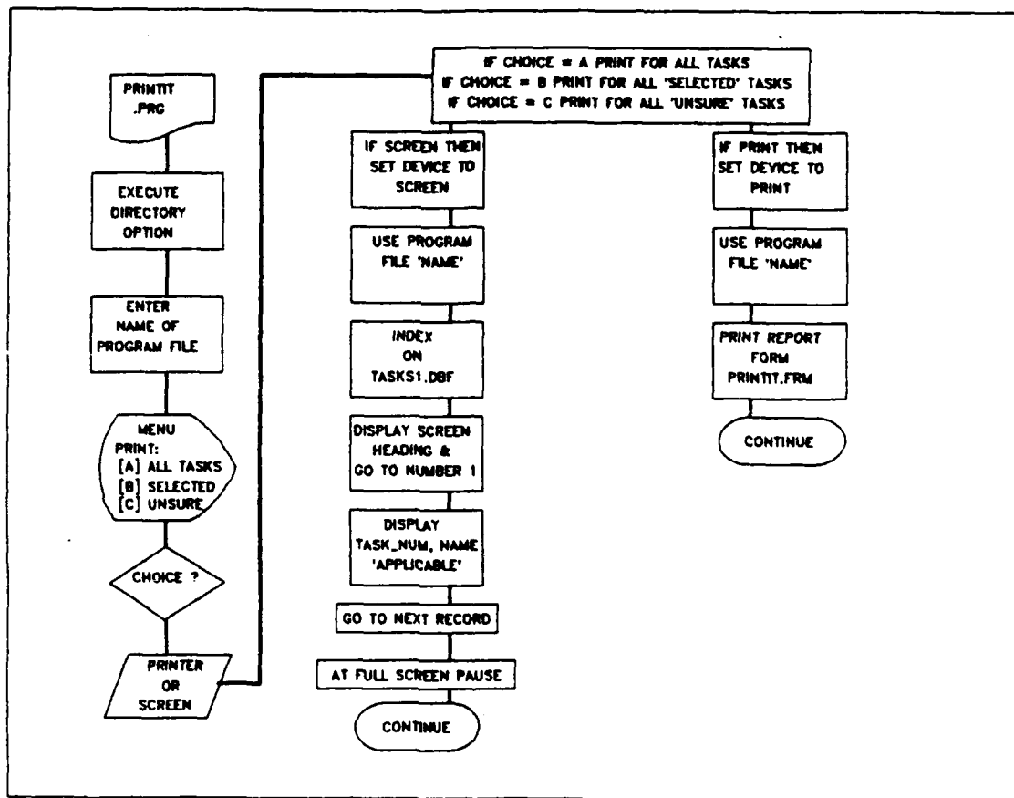
Figure 9. PRINTIT.PRG Structure
