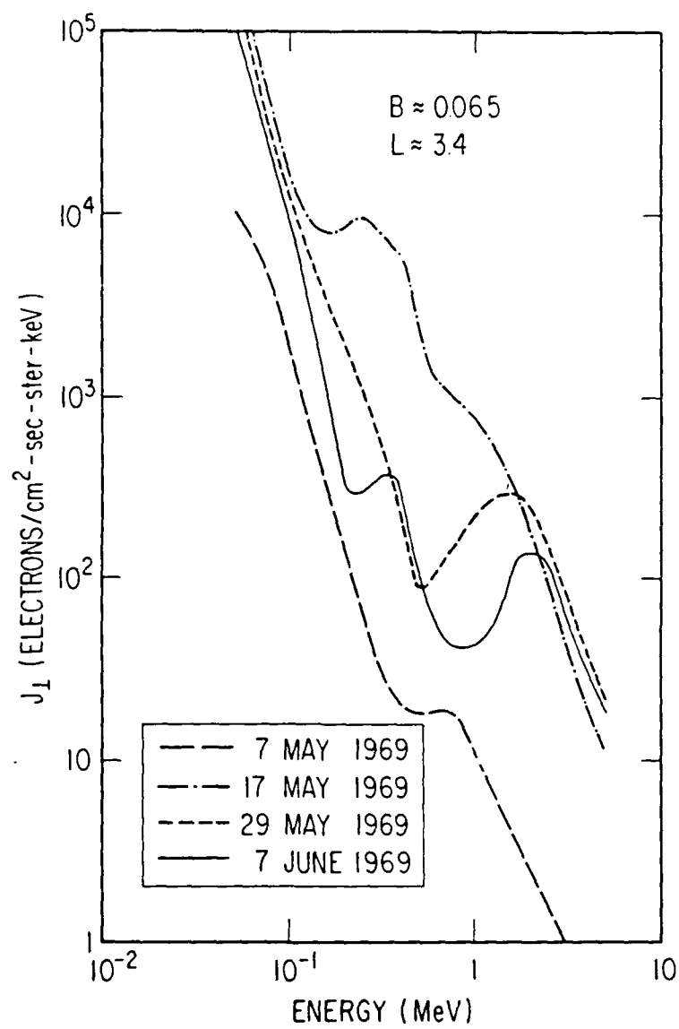
Fig. 4. Magnetic Storm-Induced Electron Flux Increases
