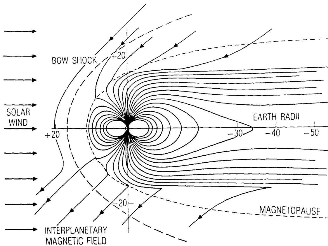
Fig. 1. Solar Wind-Geomagnetosphere Interaction Geometry
