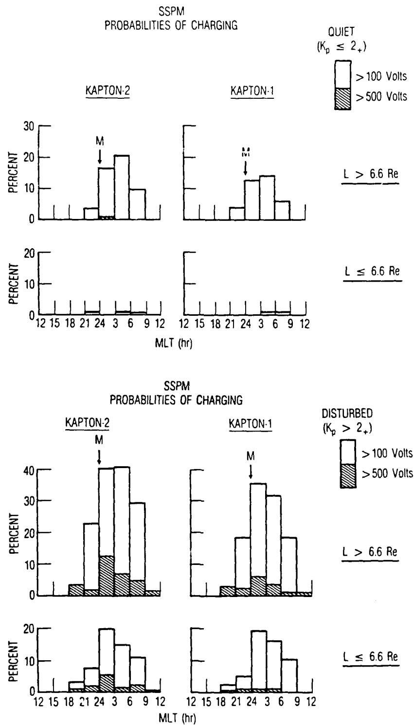
Fig. 7. Histograms of the Probabilities of Charging versus Magnetic Activity
