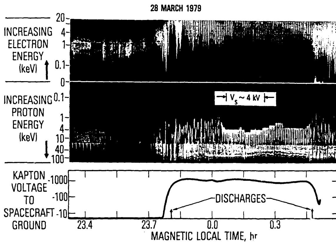
Fig. 6. Natural Charging Event on the P78-2 (SCATHA) Spacecraft in Eclipse
