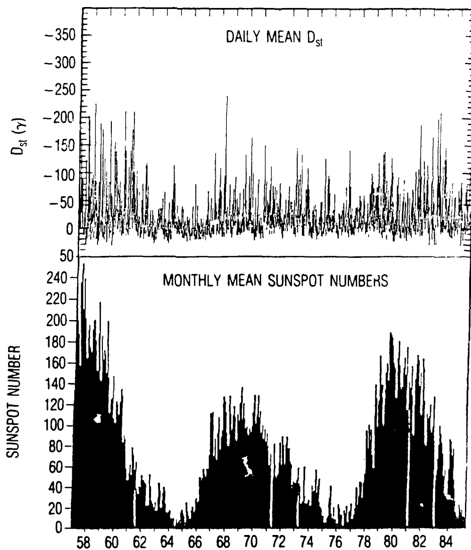
Fig. 2. Comparison of Monthly Mean Sunspot Numbers and Daily Mean D_{st} for 1957 to 1984
