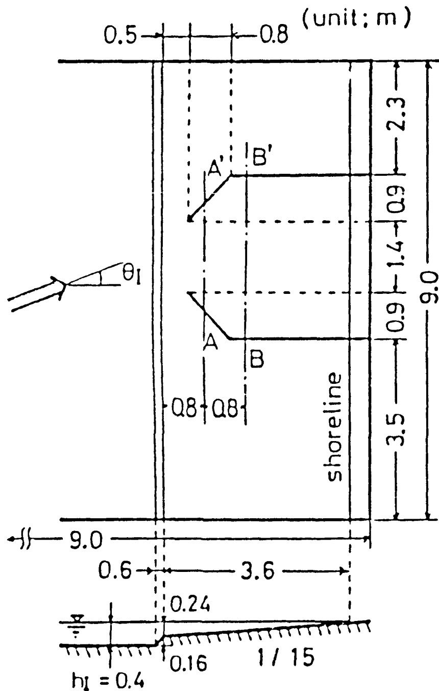
Figure 3.17 Laboratory Set-up of Two Breakwaters on a Plane Beach
