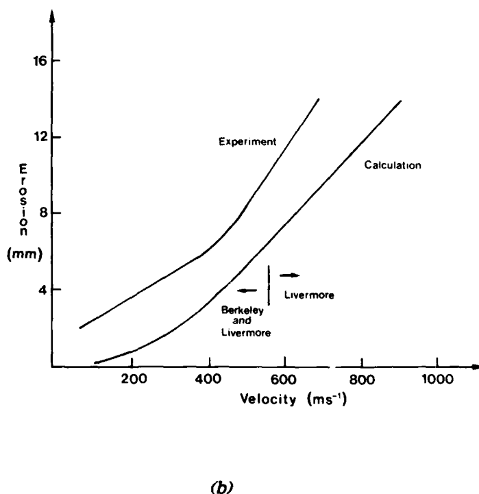
Figure 7 (a) Comparison of ballistic limit predictions using the model for thin backings with data presented by Mayseless et al. [4]. For the Livermore data, due to Wilkins [3], two values of ceramic strength have been used, 8.8 GPa corresponding to the hardness and 3.03 GPa corresponding to hardness divided by 2.9. (b) Comparison of penetrator erosion calculated using the present model with the experimental curve of Mayseless et al. [4].
