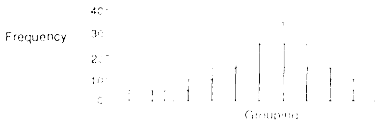
Sample Histogram
