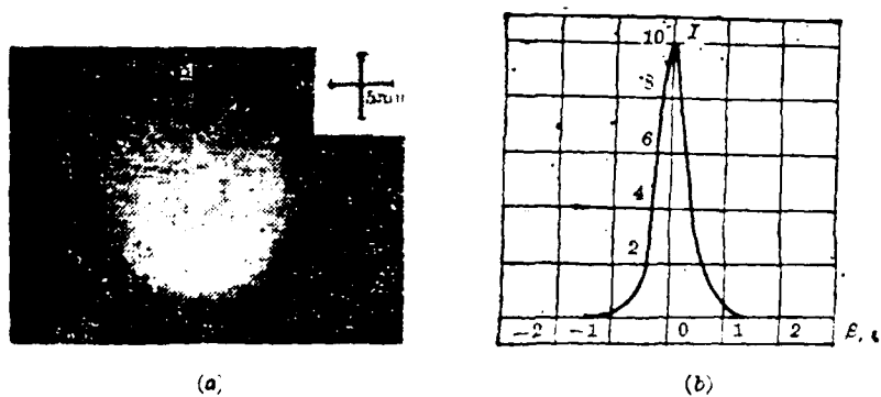
Fig. 9 (a) Gaussian light spot for v=0 ; (b) Intensity profile of light spot ( g=1, u=0, c=0.54 )
