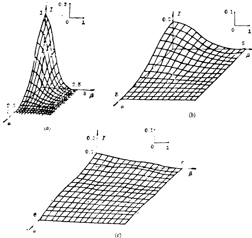
Fig. 5. Gaussian intensity distribution for \mu=0.43 . (a) \nu=0 . (b) \nu=1.5 . (c) \nu=2.5 .
