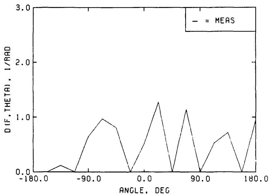
MEASURED DIRECTIONAL SPREADING CASE 70U3 -- FP=0.47, HMO=5.07, D=-9, H=1.51
