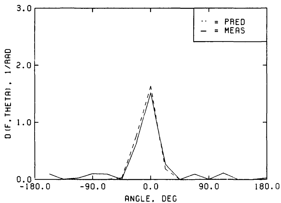
MEASURED VS PREDICTED DIRECTIONAL SPREADING CASE 72D3 -- FP=0.47, HMO=4.11, D=-11, H=1.51
