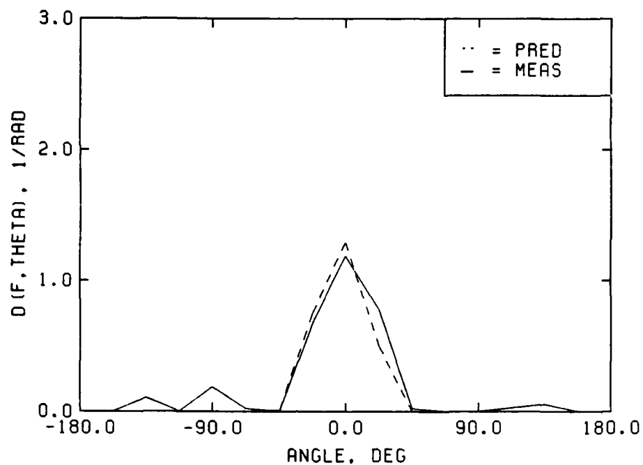
MEASURED VS PREDICTED DIRECTIONAL SPREADING CASE 70D3 -- FP=0.47, HMO=5.07, D=-2, H=1.51
