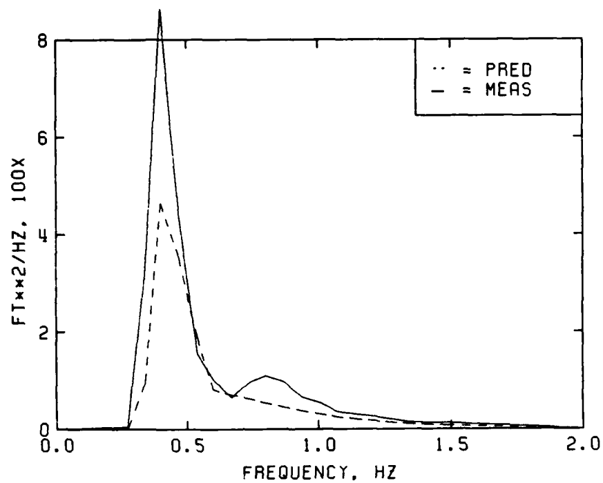
MEASURED VS PREDICTED FREQUENCY SPECTRA CASE 83U3 -- FP=0.40, HMO=4.99, H=1.51
