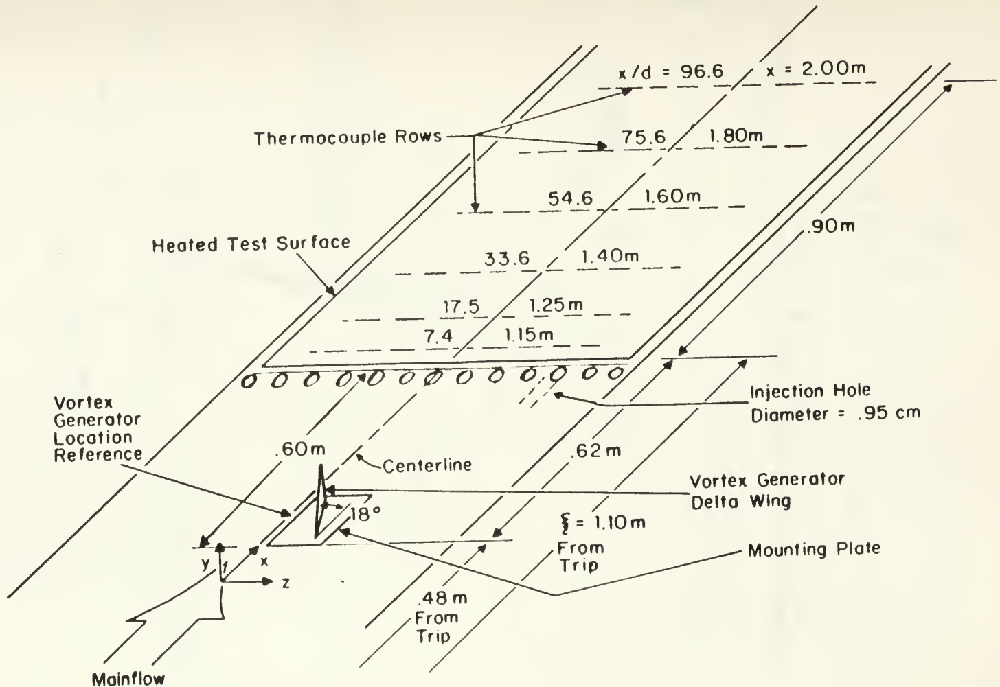
Figure 2. Top View Schematic of Wind Tunnel Test Section
