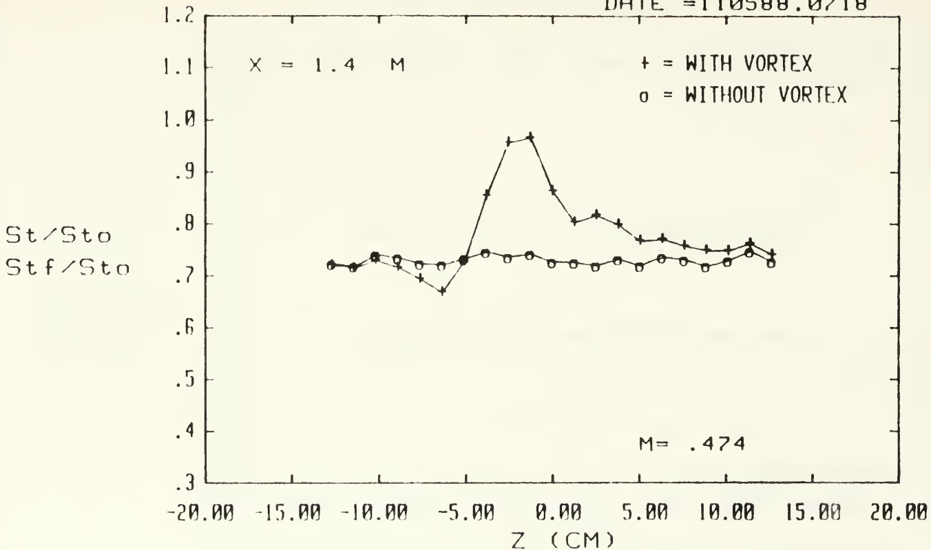
Figure 166. Spanwise Variation of St/St_0 and Stf/St_0 Ratios m=0.5 , 13 Injection Holes x/d=33.6 , Vortex r
