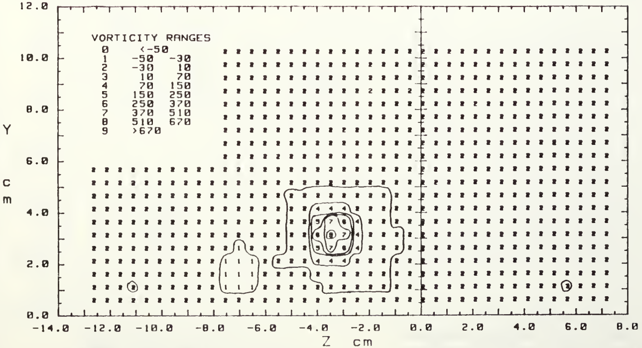
Figure 19. Streamwise Vorticity Contours, x/d=41.9 m=0.5, 13 Injection Holes, \Gamma=.111 , m^2/s , S=2.33 , Vortex W
