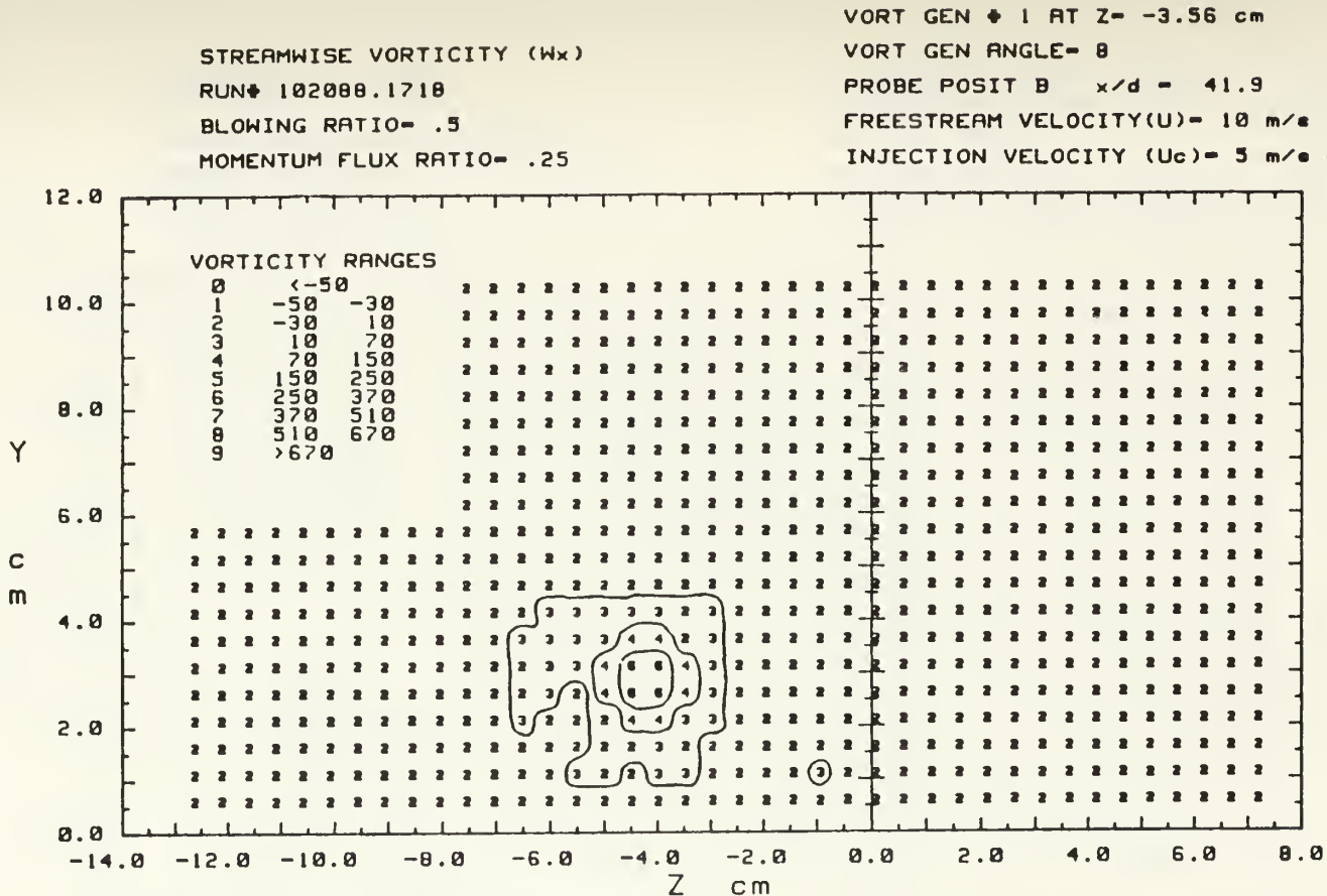
Figure 16. Streamwise Vorticity Contours, x/d=41.9 m=0.5 , Single Injection Hole \Gamma = .051 \text{ m}^2/\text{s} , S=1.08 , Vortex \gamma
