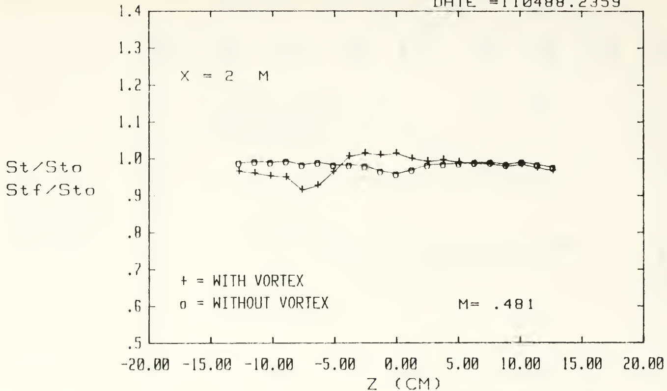
Figure 138. Spanwise Variation of St/St_0 and St_f/St_0 Ratios m=0.5 , Single Injection Hole x/d=96.6 , Vortex 2
