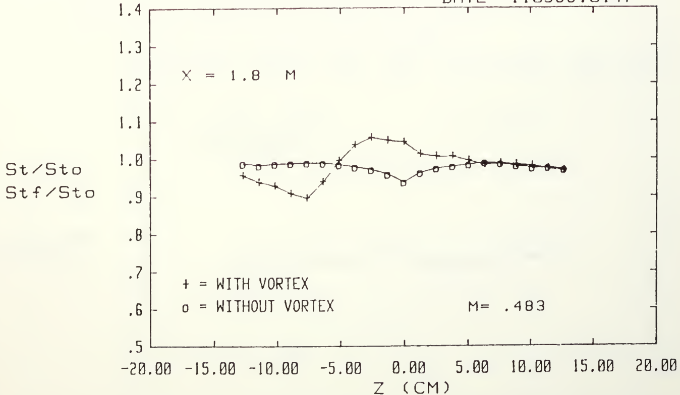
Figure 133. Spanwise Variation of St/St_0 and St_f/St_0 Ratios M=0.5 , Single Injection Hole x/d=75.6 , Vortex \gamma
