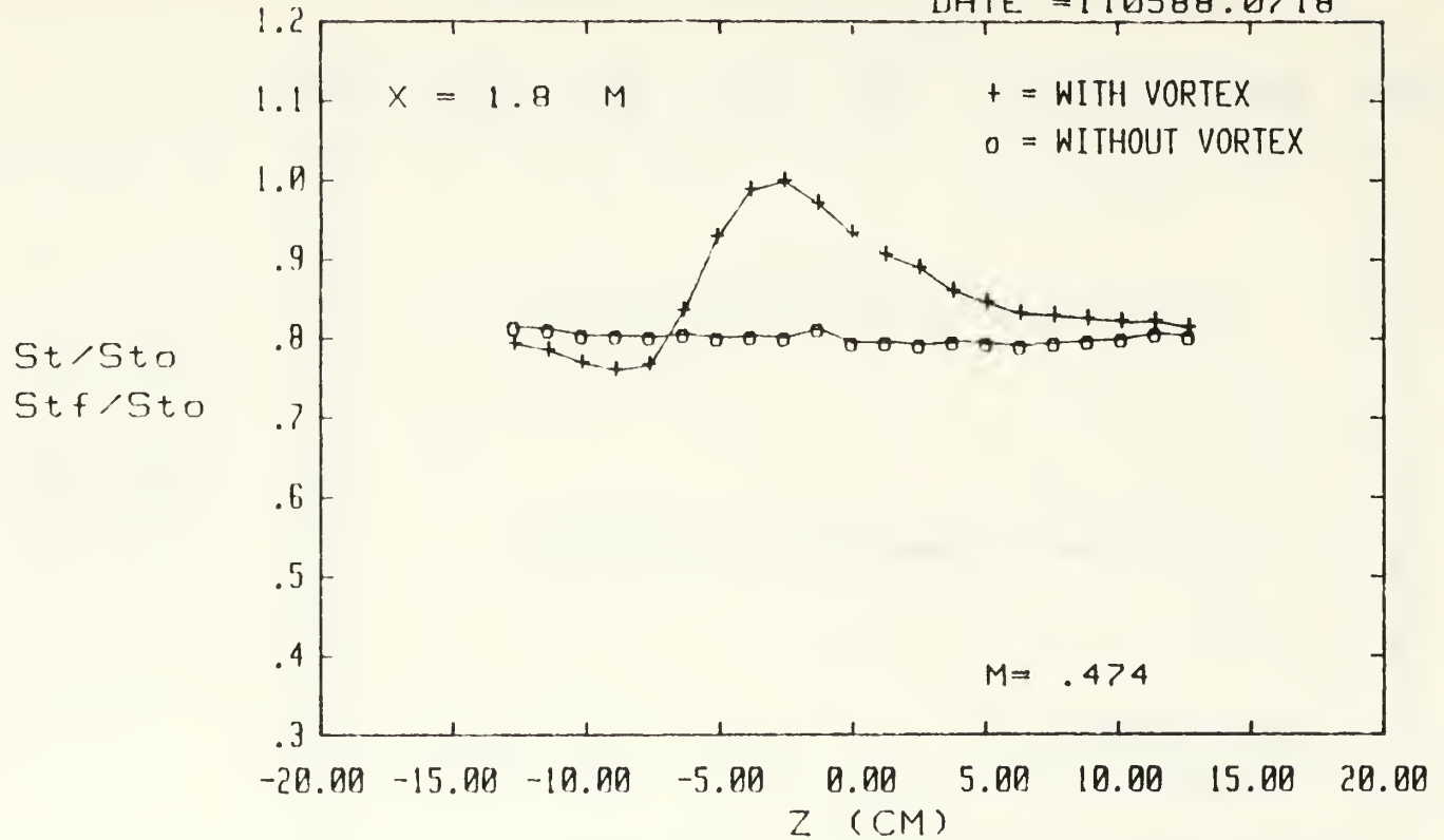
Figure 178. Spanwise Variation of St/St_0 and Stf/St_0 Ratios m=0.5 , 13 Injection Holes x/d=75.6 , Vortex r
