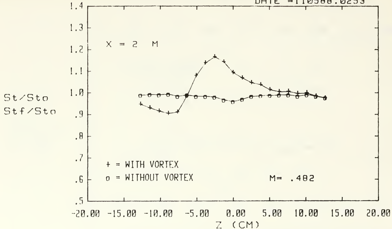
Figure 140. Spanwise Variation of St/St_0 and Stf/St_0 Ratios m=0.5 , Single Injection Hole x/d=96.6 , Vortex x
