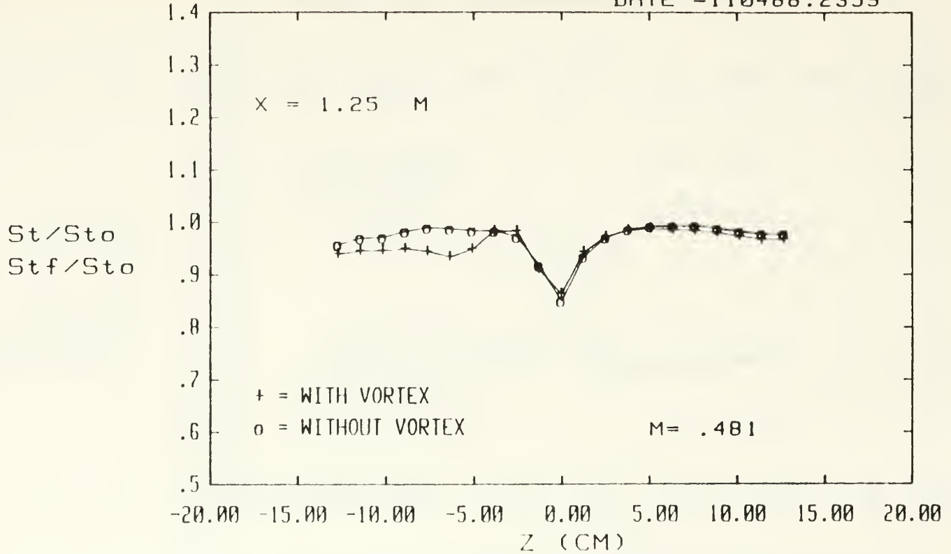
Figure 114. Spanwise Variation of St/Sto and Stf/Sto Ratios M=0.5 , Single Injection Hole x/d=17.5 , Vortex z
