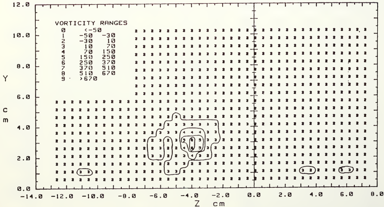
Figure 21. Streamwise Vorticity Contours, x/d=41.9 m=0.5 , 13 Injection Holes, \Gamma = .042 \text{ m}^2/\text{s} , S=0.89 , Vortex Y
