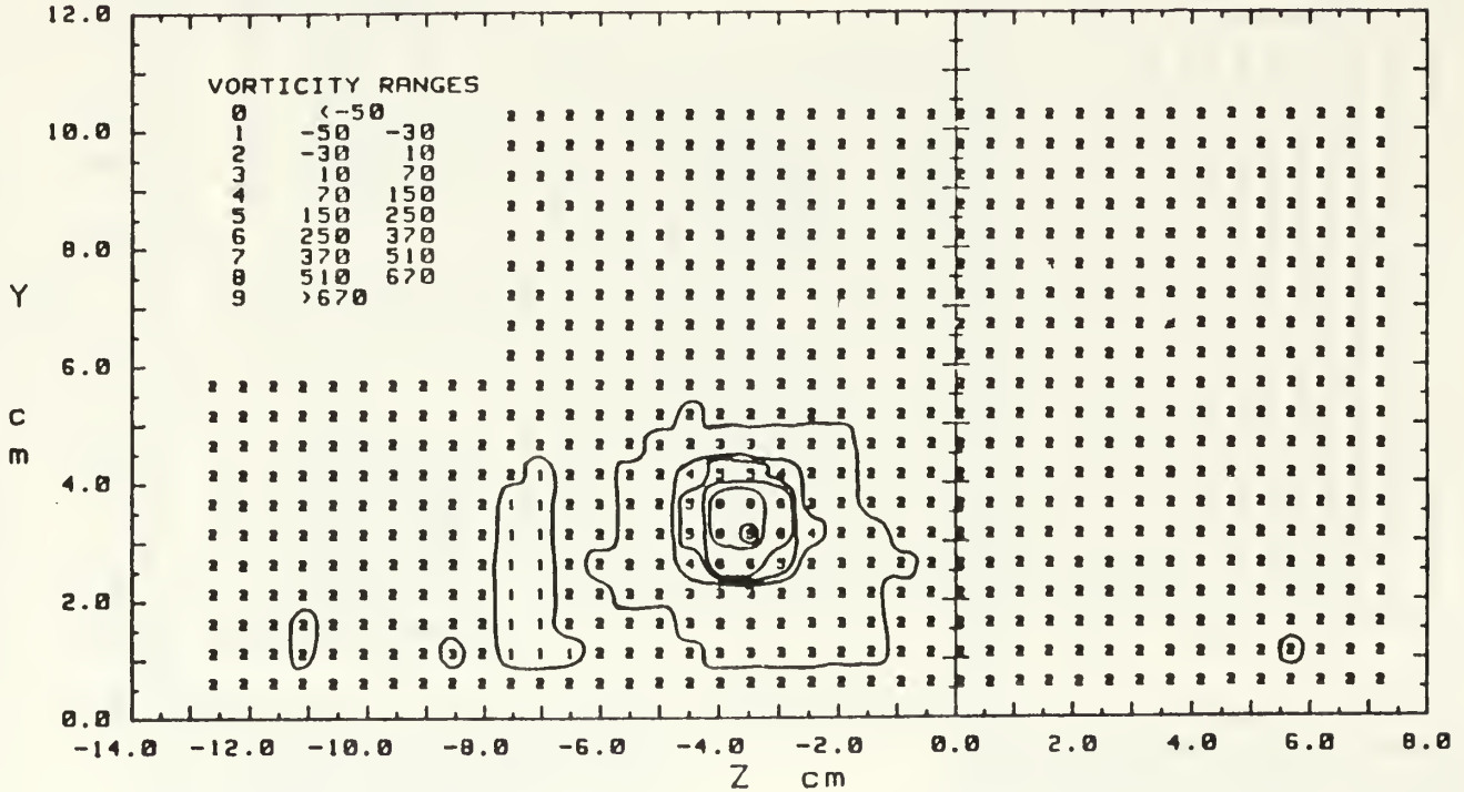
Figure 18. Streamwise Vorticity Contours, X.d=41.9 m=0.5, 13 Injection Holes, \Gamma = .134 m 2 /s, S=2.81, Vortex \Gamma
