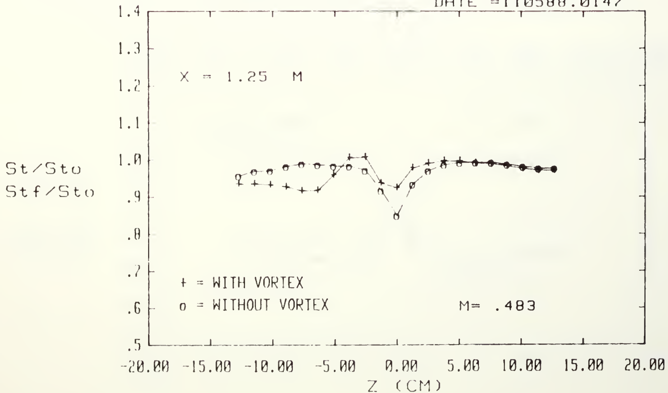
Figure 115. Spanwise Variation of St/St_0 and St_f/St_0 Ratios m=0.5 , Single Injection Hole x/d=17.5 , Vortex \gamma
