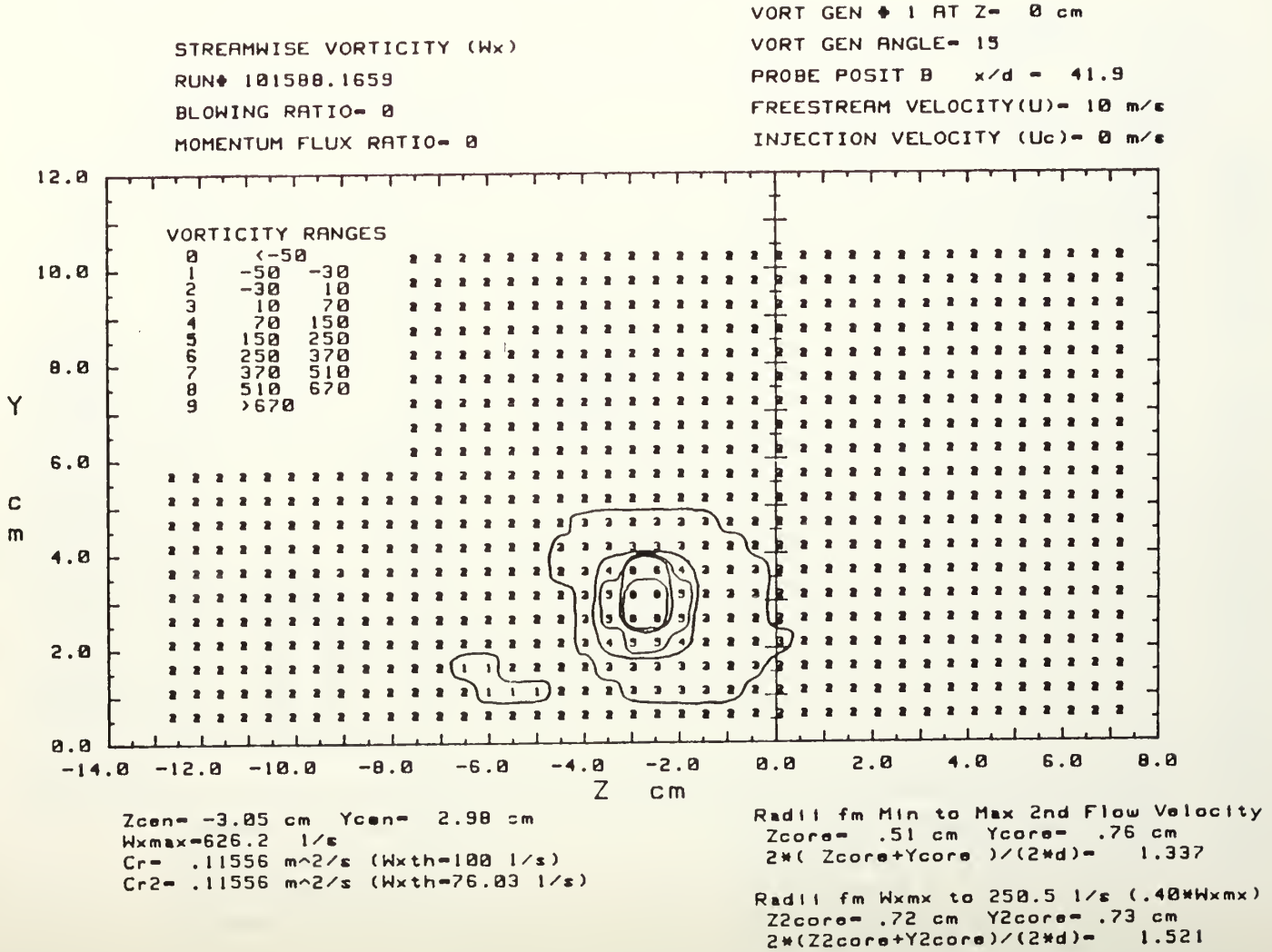
Figure 9. Streamwise Vorticity Contours, m=0 x/d=41.9 , \Gamma = .115 \text{ m}^2/\text{s} , Vortex 5
