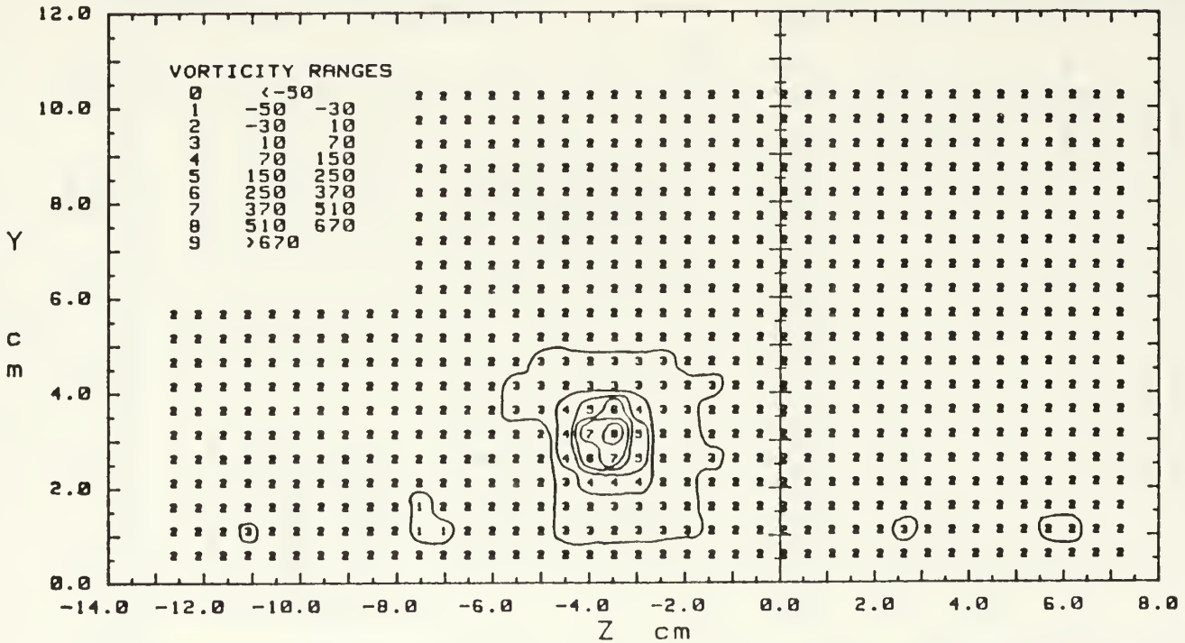
Figure 20. Streamwise Vorticity Contours, x/d=41.9 m=0.5 , 13 Injection Holes, \Gamma = .088 \text{ m}^2/\text{s} , S=1.86 , Vortex x
