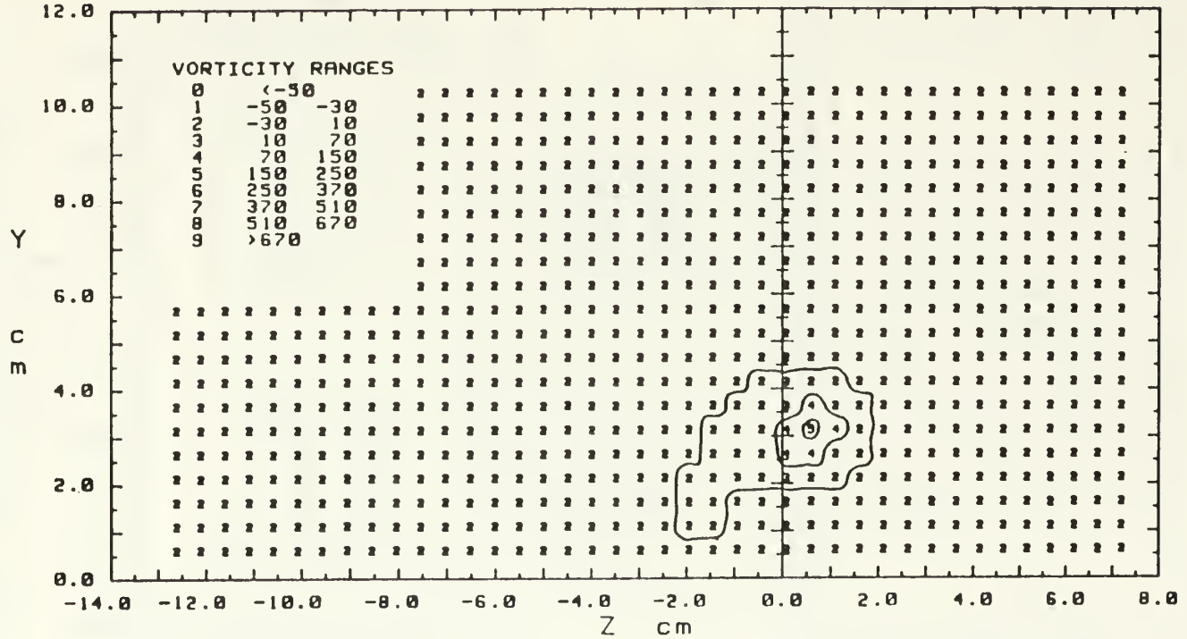
Figure 12. Streamwise Vorticity Contours, M=0 x/d=41.9 \Gamma=0.019 m 2 /s, Vortex v
