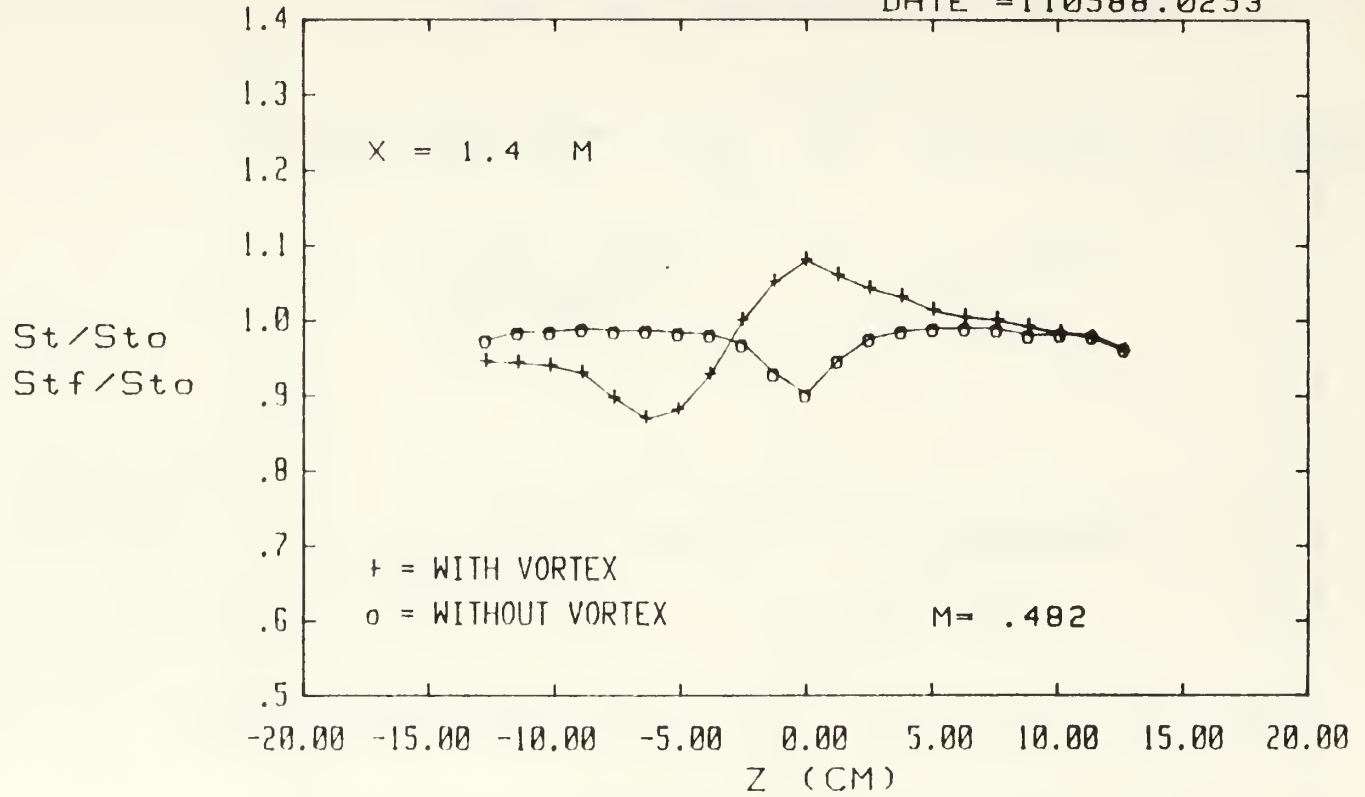
Figure 122. Spanwise Variation of St/St_0 and Stf/St_0 Ratios m=0.5 , Single Injection Hole x/d=33.6 , Vortex x
