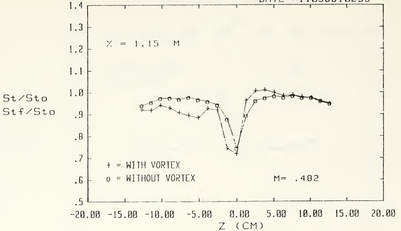
Figure 110. Spanwise Variation of St/St_0 and St_f/St_0 Ratios m=0.5 , Single Injection Hole x/d=7.4 , Vortex x
