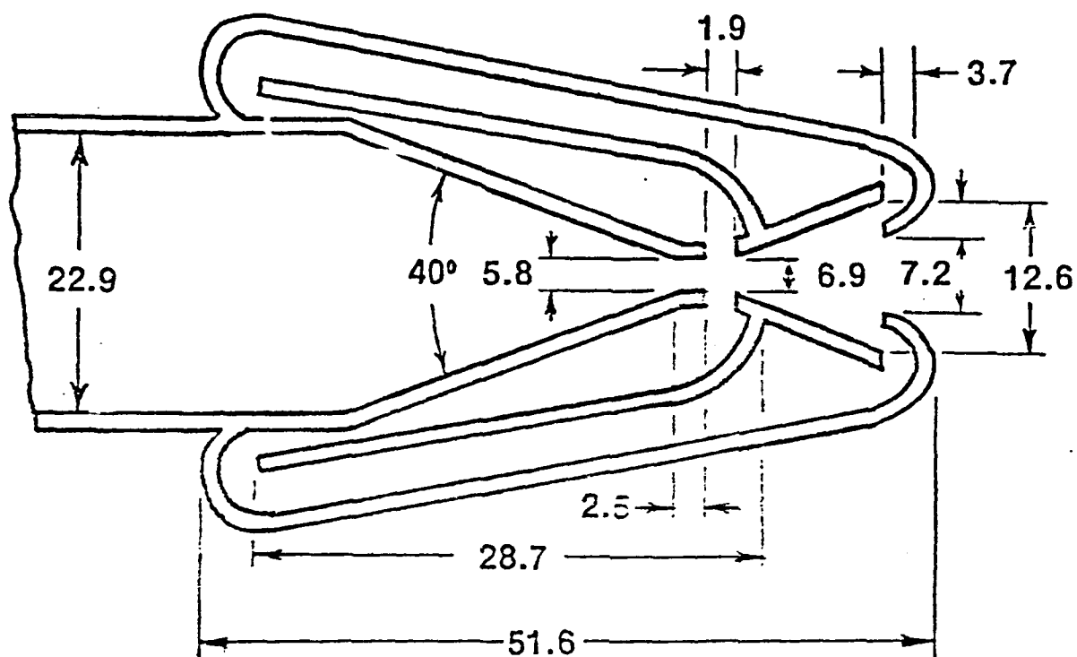
Nozzle 2 dimensions in millimeters
