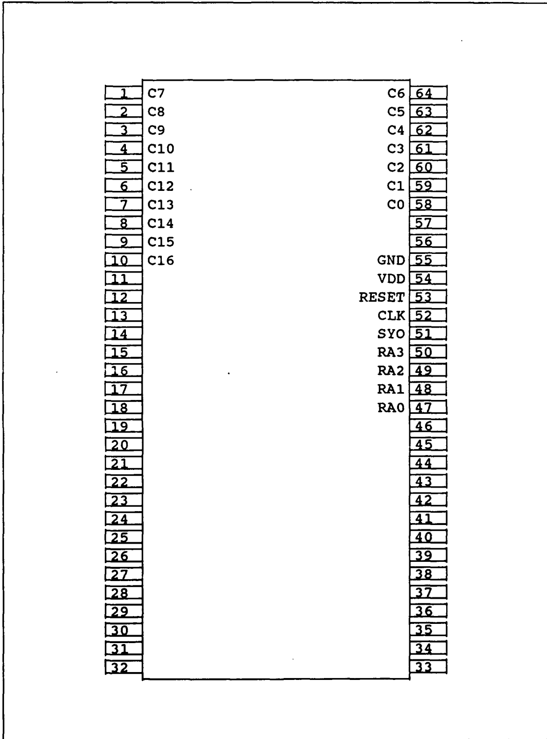
Figure 12. Wire bonding Diagram for Redesigned Brain Chip
