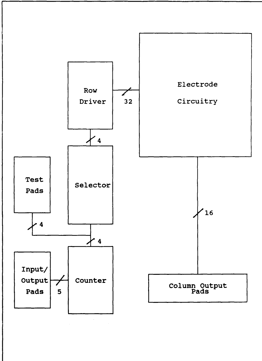
Figure 3. Block Diagram of the New Brain Chip
