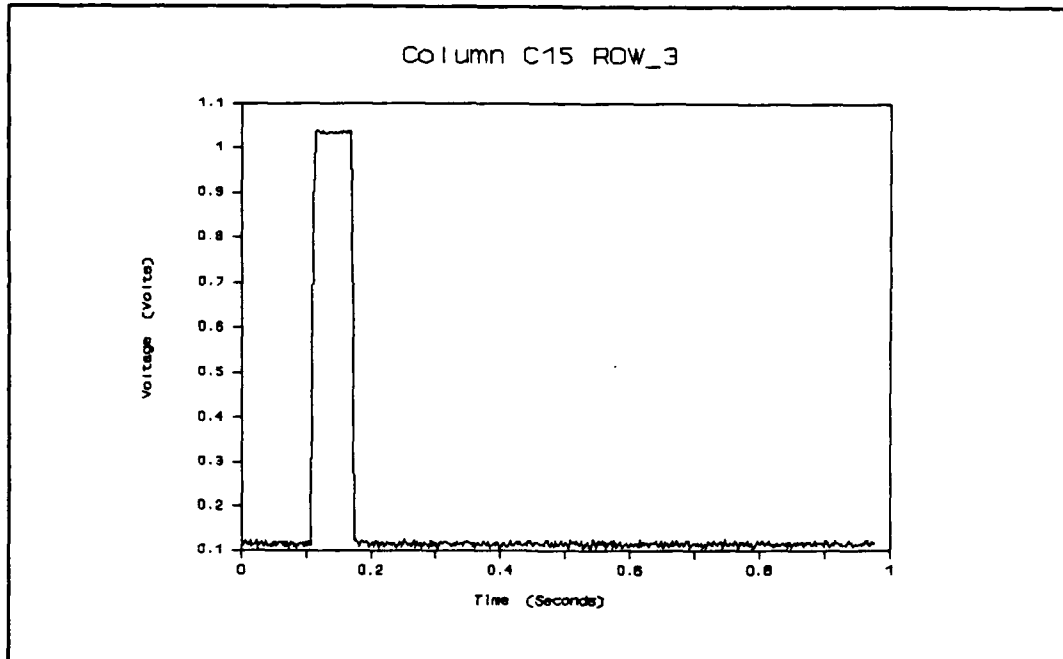
Figure 15. Output of Column C15 with 1-Volt Applied to ROW_3
