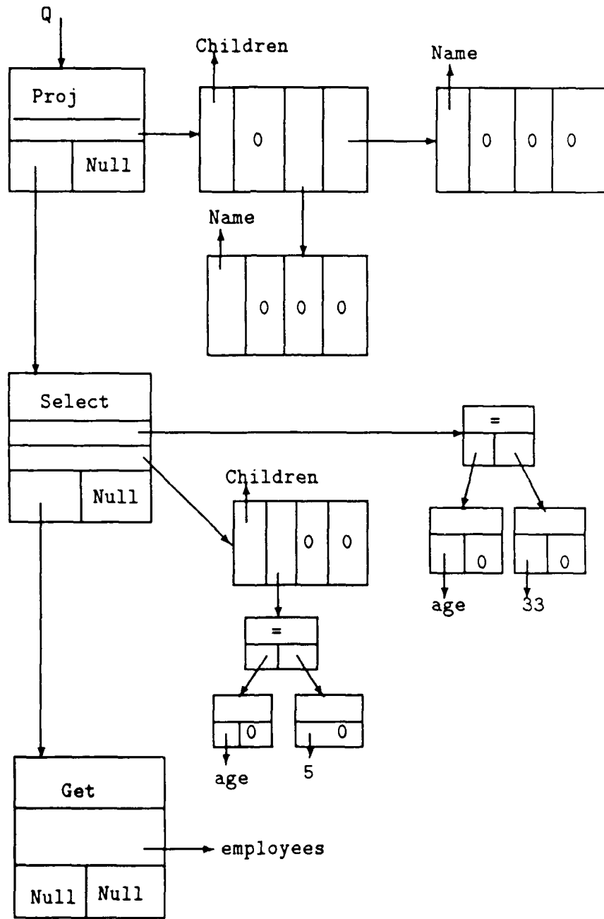
Figure 4.11. A query tree structure.
