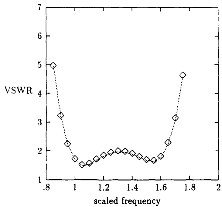
Figure 4.26. Plot of VSWR versus Scaled Frequency for the Open-Sleeve Dipole with l_2 = 0.28\lambda , s = 0.02\lambda , and Z_0 = 150\Omega
