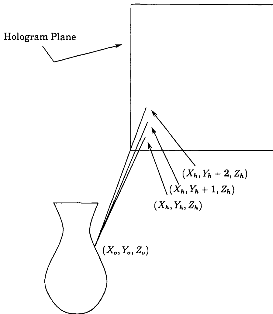
Figure 10. Front View of the Problem Geometry
