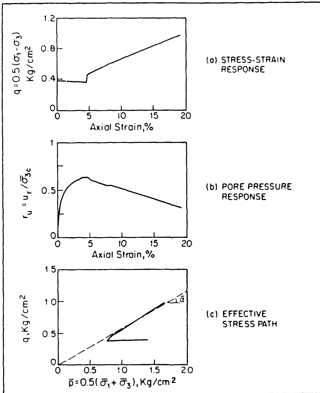
Fig. 6.46. Results of a CyT- \overline{\text{CAU}} Test on a Dilative Sample of Sand SF7 Carried Out Until It Reached the Strength Envelope \bar{\alpha} = \bar{\alpha}_{us} = 29^\circ followed by Monotonic Loading (CyT- \overline{\text{CAU}} + \overline{\text{CAU}} Test)
