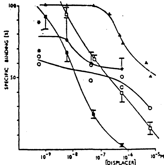
Figure 1. Effect of unlabelled 1 (●), 4- t -butyl-1-(4-ethynylphenyl)-2,6,7-trioxabicyclo[2.2.2]octane (○), picrotoxinin (▲), lindane (■) and ivermectin (○) on specific binding of [ 3 H]- 1 to cockroach CNS. Dieldrin gave 16±2% and 30±3% displacement of [ 3 H]- 1 at 60nM and 0.6μM respectively.
